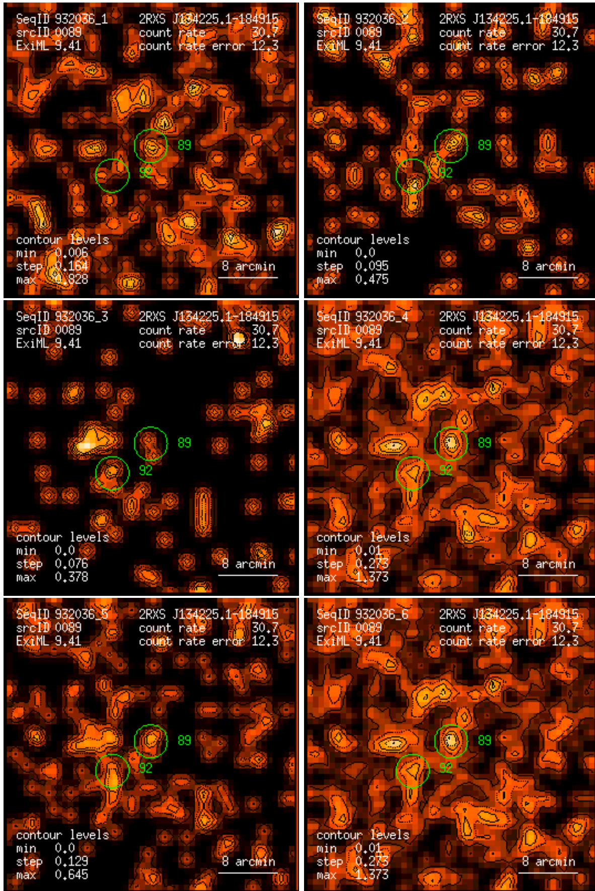
Figure 89: RASS 932036: detection 0089: band rate images, Gaussian filter: (1) PSPC channels 11 – 41, (2) 52 – 90, (3) 91 – 201, (4) 11 – 235, (5) 52 – 201, (6) 11 – 201. Broad band rates in counts/ks. Band rate contour levels in counts/ks/arcmin 2 .
