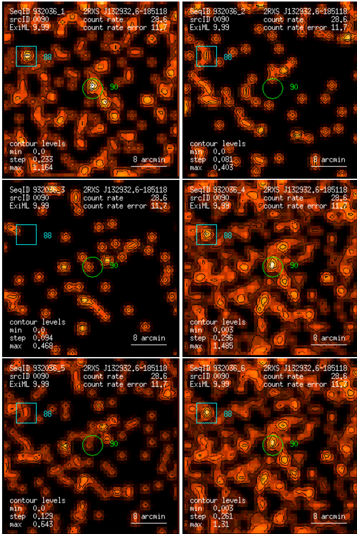
Figure 90: RASS 932036: detection 0090: band rate images, Gaussian filter: (1) PSPC channels 11 – 41, (2) 52 – 90, (3) 91 – 201, (4) 11 – 235, (5) 52 – 201, (6) 11 – 201. Broad band rates in counts/ks. Band rate contour levels in counts/ks/arcmin 2 .
