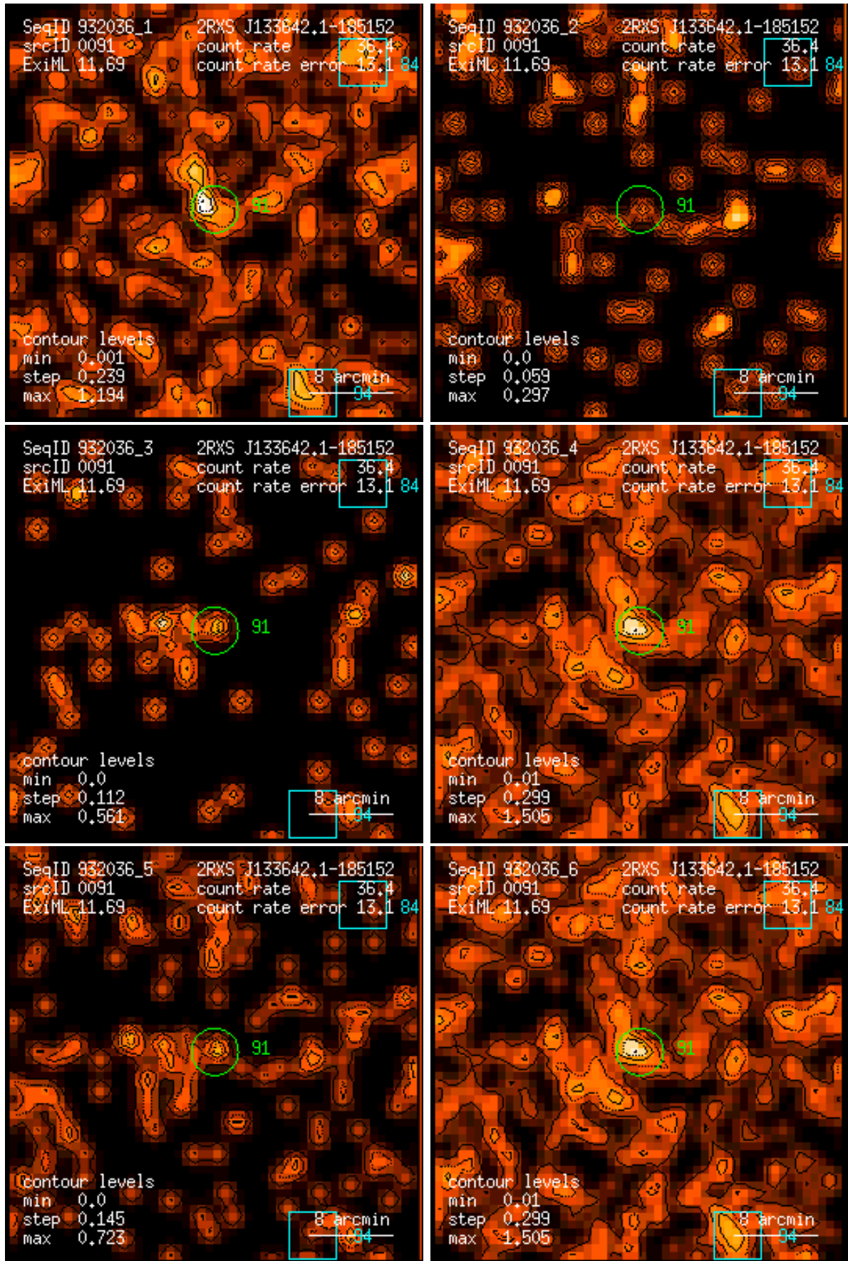
Figure 91: RASS 932036: detection 0091: band rate images, Gaussian filter: (1) PSPC channels 11 – 41, (2) 52 – 90, (3) 91 – 201, (4) 11 – 235, (5) 52 – 201, (6) 11 – 201. Broad band rates in counts/ks. Band rate contour levels in counts/ks/arcmin 2 .
