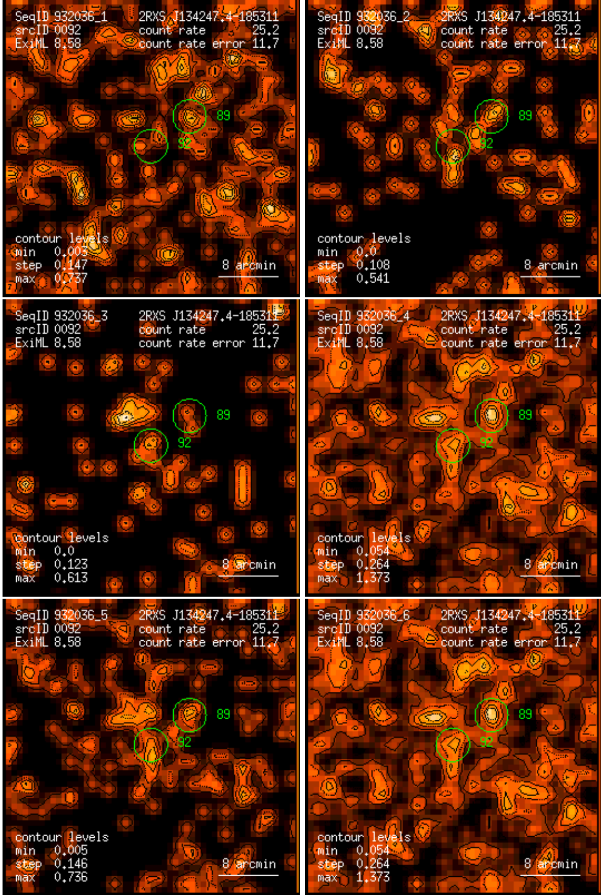
Figure 92: RASS 932036: detection 0092: band rate images, Gaussian filter: (1) PSPC channels 11 – 41, (2) 52 – 90, (3) 91 – 201, (4) 11 – 235, (5) 52 – 201, (6) 11 – 201. Broad band rates in counts/ks. Band rate contour levels in counts/ks/arcmin 2 .
