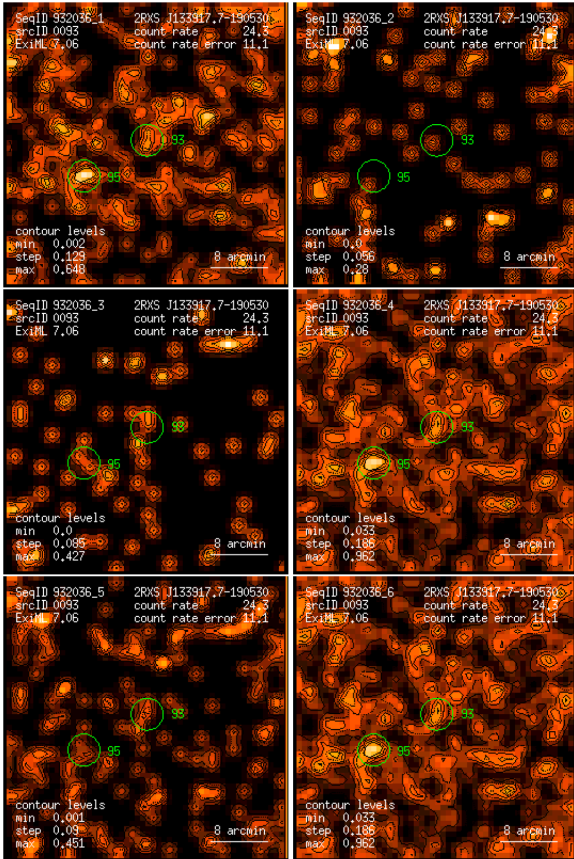
Figure 93: RASS 932036: detection 0093: band rate images, Gaussian filter: (1) PSPC channels 11 – 41, (2) 52 – 90, (3) 91 – 201, (4) 11 – 235, (5) 52 – 201, (6) 11 – 201. Broad band rates in counts/ks. Band rate contour levels in counts/ks/arcmin 2 .
