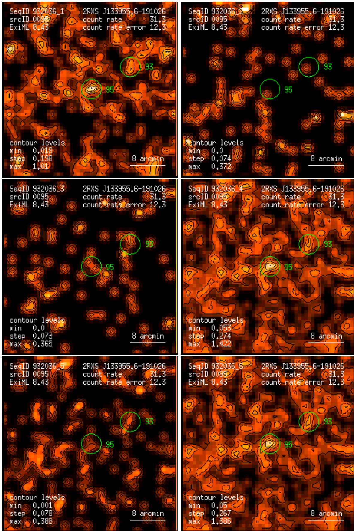
Figure 95: RASS 932036: detection 0095: band rate images, Gaussian filter: (1) PSPC channels 11 – 41, (2) 52 – 90, (3) 91 – 201, (4) 11 – 235, (5) 52 – 201, (6) 11 – 201. Broad band rates in counts/ks. Band rate contour levels in counts/ks/arcmin 2 .
