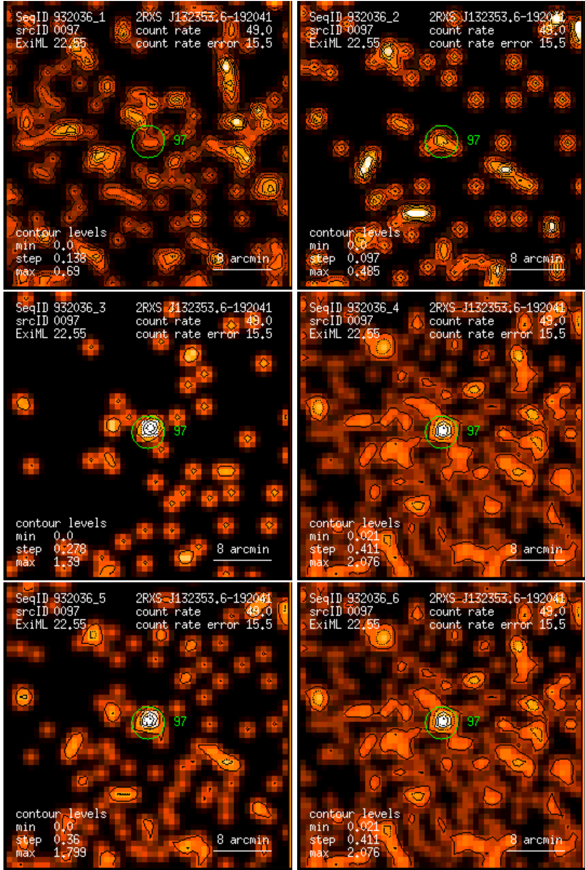
Figure 97: RASS 932036: detection 0097: band rate images, Gaussian filter: (1) PSPC channels 11 – 41, (2) 52 – 90, (3) 91 – 201, (4) 11 – 235, (5) 52 – 201, (6) 11 – 201. Broad band rates in counts/ks. Band rate contour levels in counts/ks/arcmin 2 .
