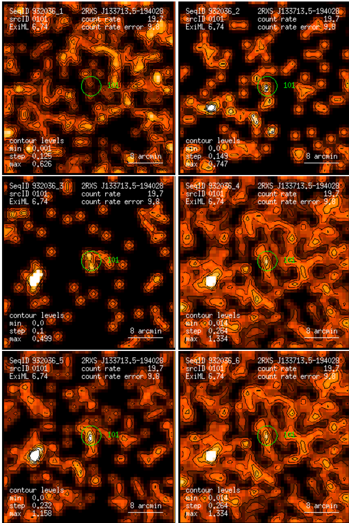
Figure 101: RASS 932036: detection 0101: band rate images, Gaussian filter: (1) PSPC channels 11 – 41, (2) 52 – 90, (3) 91 – 201, (4) 11 – 235, (5) 52 – 201, (6) 11 – 201. Broad band rates in counts/ks. Band rate contour levels in counts/ks/arcmin 2 .
