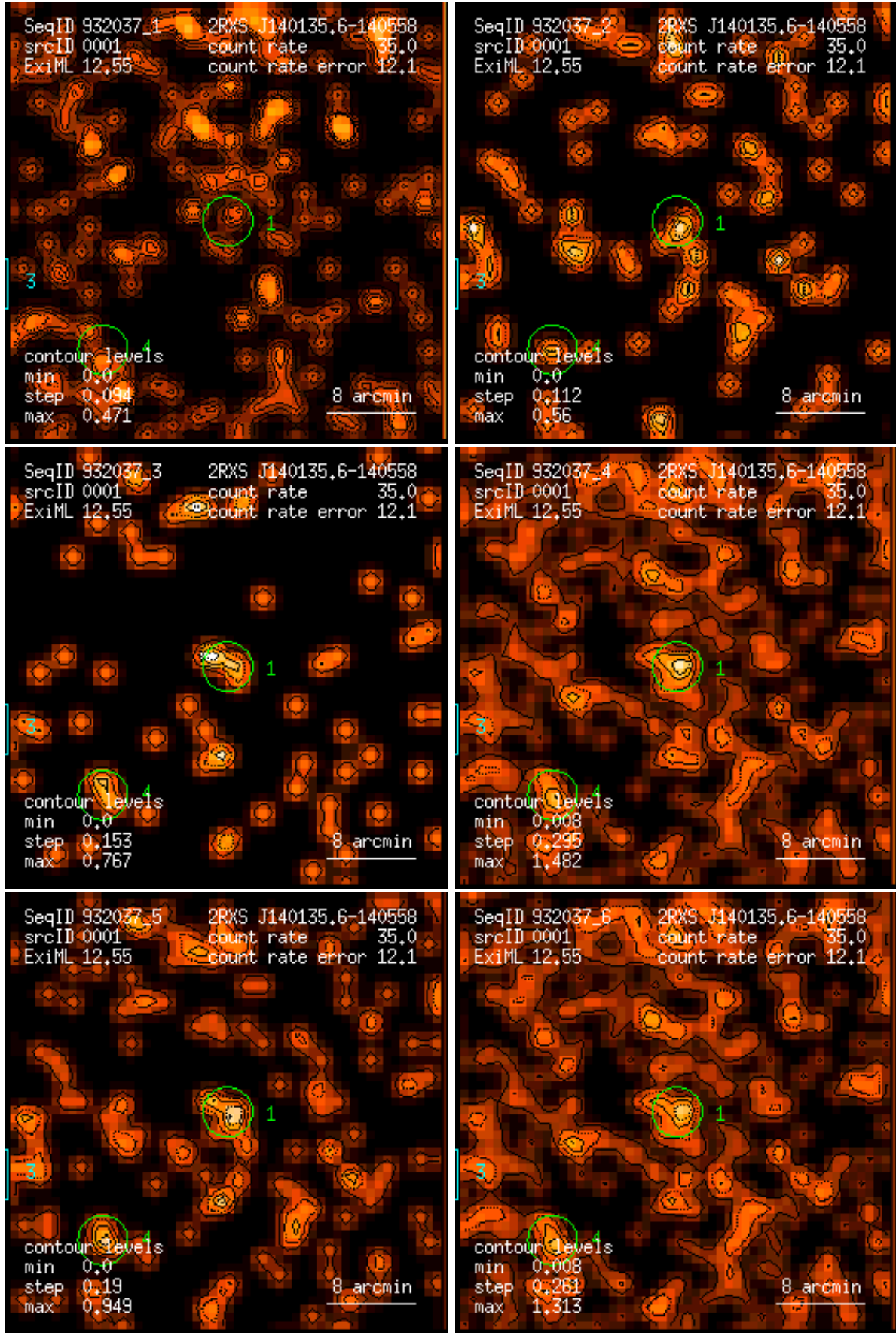
Figure 1: RASS 932037: detection 0001: band rate images, Gaussian filter: (1) PSPC channels 11 – 41, (2) 52 – 90, (3) 91 – 201, (4) 11 – 235, (5) 52 – 201, (6) 11 – 201. Broad band rates in counts/ks. Band rate contour levels in counts/ks/arcmin 2 .
