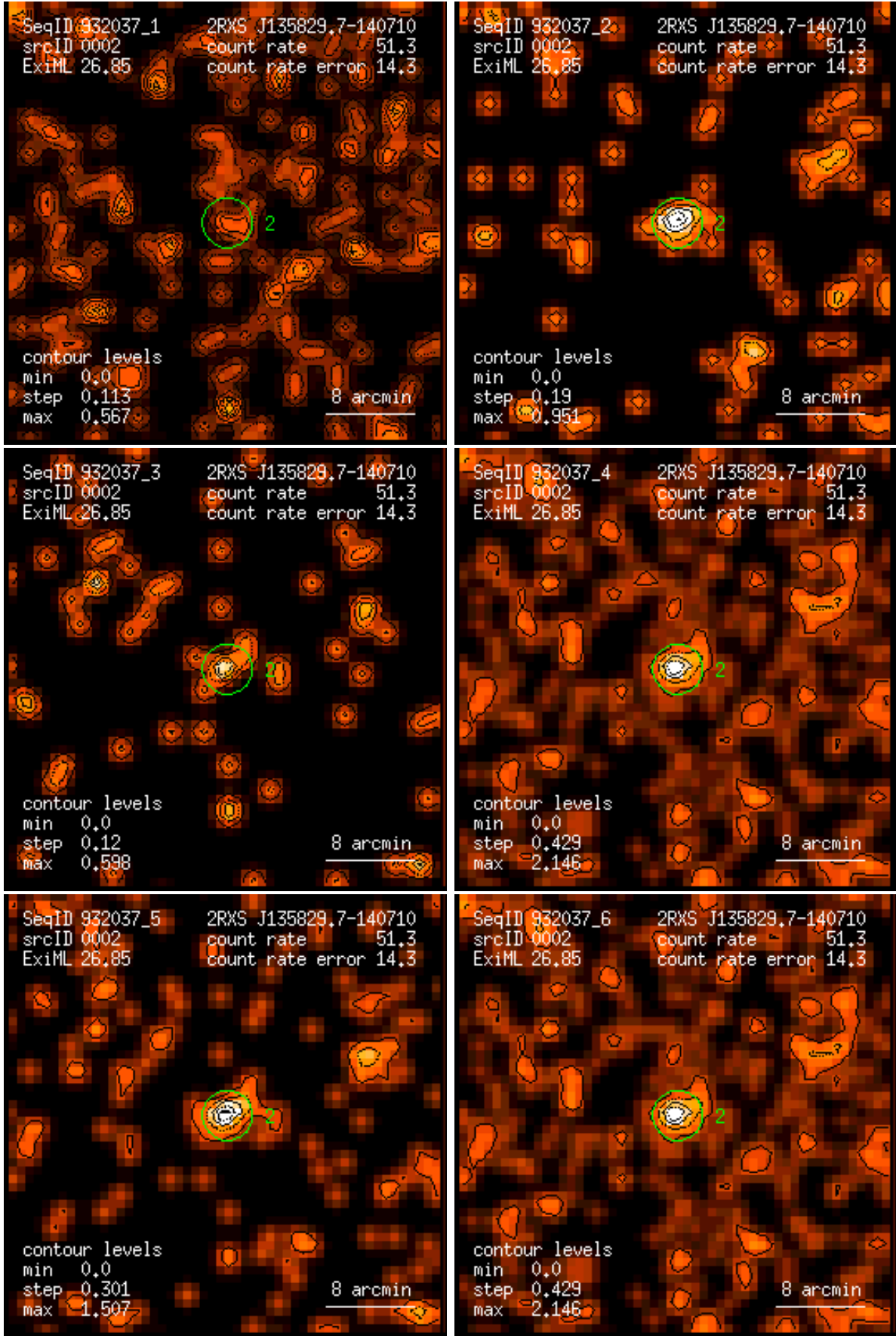
Figure 2: RASS 932037: detection 0002: band rate images, Gaussian filter: (1) PSPC channels 11 – 41, (2) 52 – 90, (3) 91 – 201, (4) 11 – 235, (5) 52 – 201, (6) 11 – 201. Broad band rates in counts/ks. Band rate contour levels in counts/ks/arcmin 2 .
