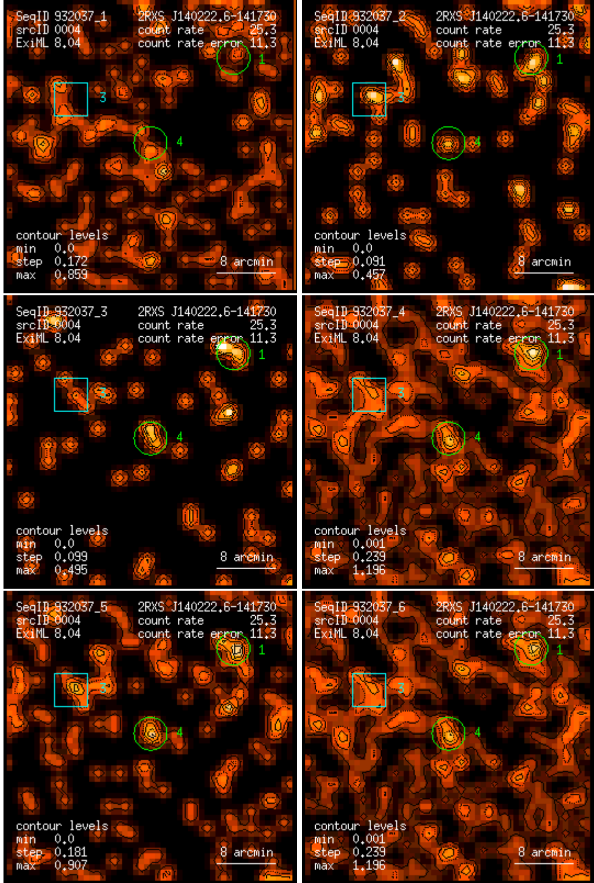
Figure 4: RASS 932037: detection 0004: band rate images, Gaussian filter: (1) PSPC channels 11 – 41, (2) 52 – 90, (3) 91 – 201, (4) 11 – 235, (5) 52 – 201, (6) 11 – 201. Broad band rates in counts/ks. Band rate contour levels in counts/ks/arcmin 2 .
