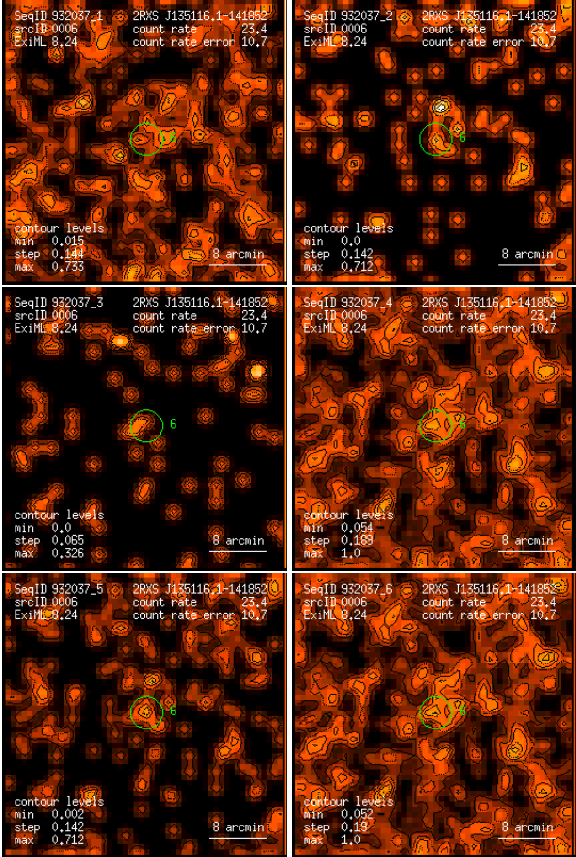
Figure 6: RASS 932037: detection 0006: band rate images, Gaussian filter: (1) PSPC channels 11 – 41, (2) 52 – 90, (3) 91 – 201, (4) 11 – 235, (5) 52 – 201, (6) 11 – 201. Broad band rates in counts/ks. Band rate contour levels in counts/ks/arcmin 2 .
