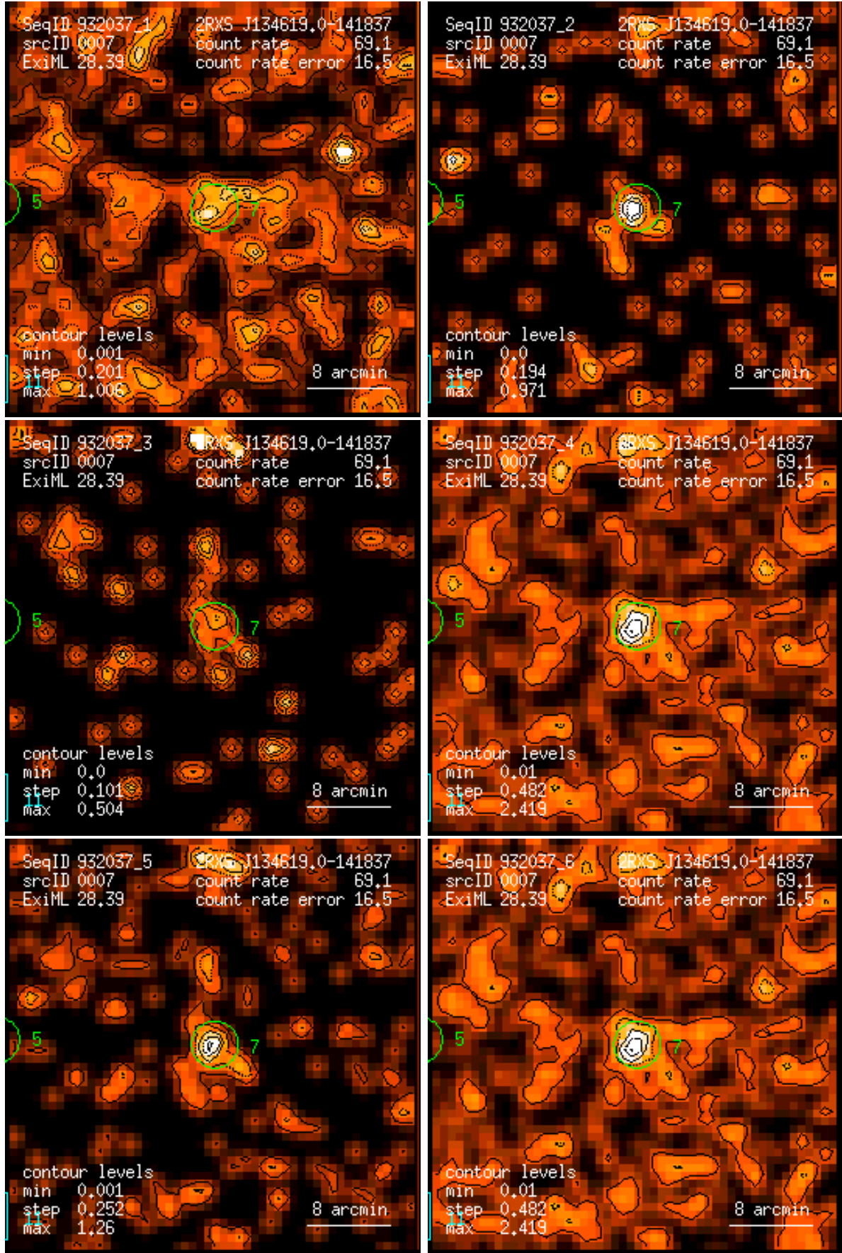
Figure 7: RASS 932037: detection 0007: band rate images, Gaussian filter: (1) PSPC channels 11 – 41, (2) 52 – 90, (3) 91 – 201, (4) 11 – 235, (5) 52 – 201, (6) 11 – 201. Broad band rates in counts/ks. Band rate contour levels in counts/ks/arcmin 2 .
