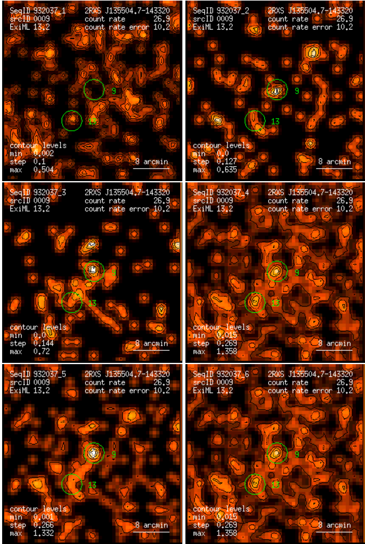
Figure 9: RASS 932037: detection 0009: band rate images, Gaussian filter: (1) PSPC channels 11 – 41, (2) 52 – 90, (3) 91 – 201, (4) 11 – 235, (5) 52 – 201, (6) 11 – 201. Broad band rates in counts/ks. Band rate contour levels in counts/ks/arcmin 2 .
