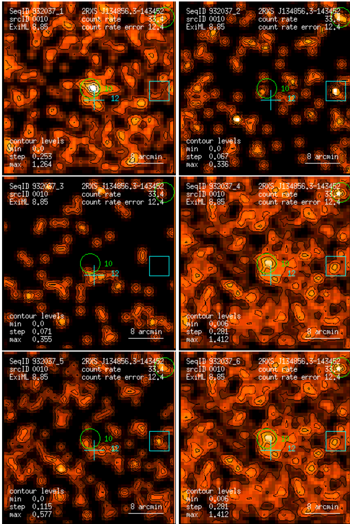
Figure 10: RASS 932037: detection 0010: band rate images, Gaussian filter: (1) PSPC channels 11 – 41, (2) 52 – 90, (3) 91 – 201, (4) 11 – 235, (5) 52 – 201, (6) 11 – 201. Broad band rates in counts/ks. Band rate contour levels in counts/ks/arcmin 2 .
