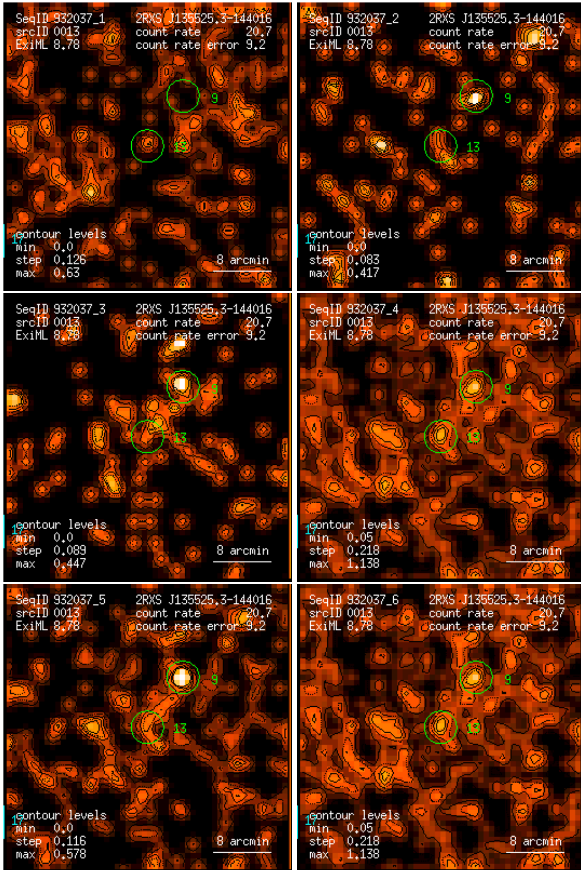
Figure 13: RASS 932037: detection 0013: band rate images, Gaussian filter: (1) PSPC channels 11 – 41, (2) 52 – 90, (3) 91 – 201, (4) 11 – 235, (5) 52 – 201, (6) 11 – 201. Broad band rates in counts/ks. Band rate contour levels in counts/ks/arcmin 2 .
