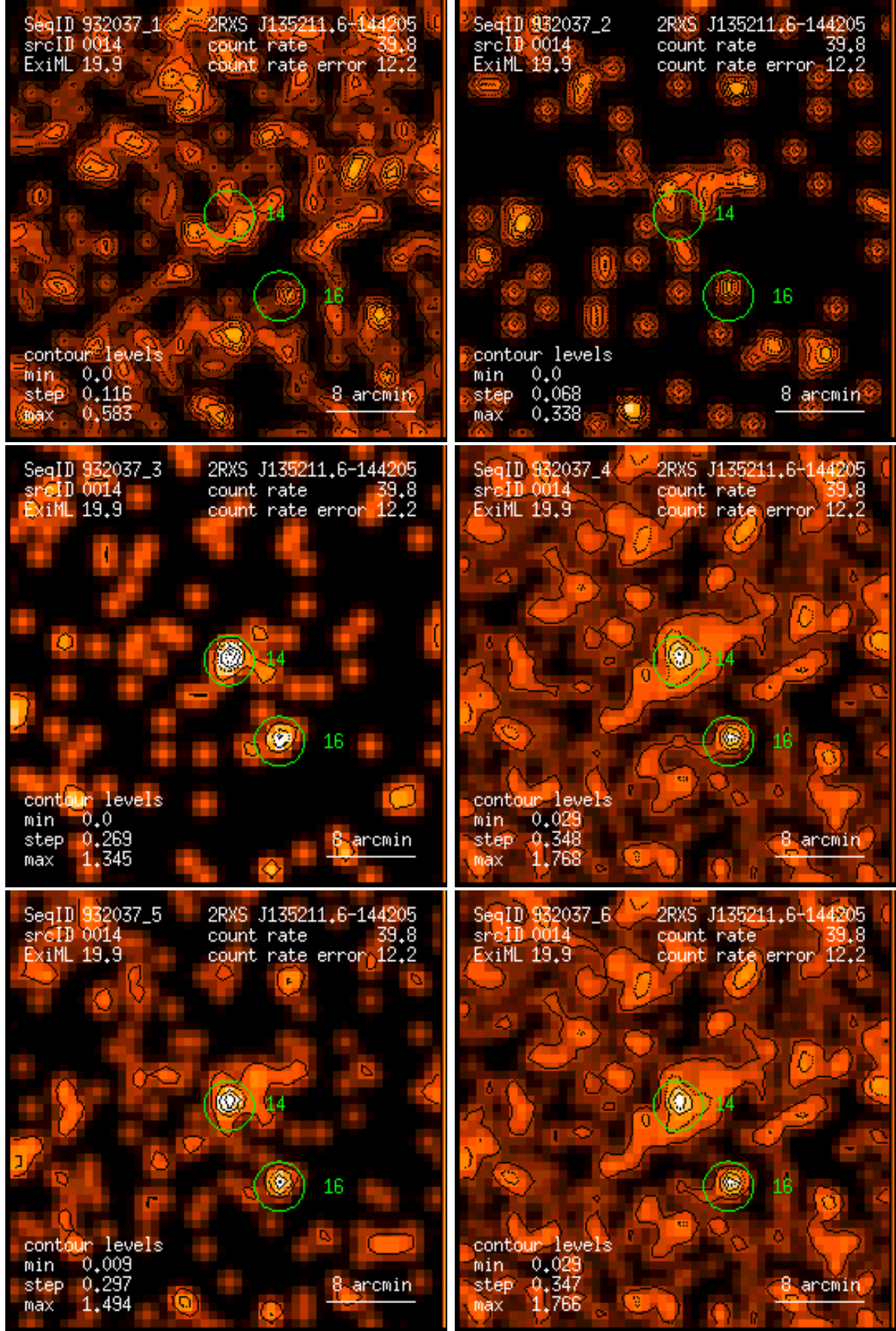
Figure 14: RASS 932037: detection 0014: band rate images, Gaussian filter: (1) PSPC channels 11 – 41, (2) 52 – 90, (3) 91 – 201, (4) 11 – 235, (5) 52 – 201, (6) 11 – 201. Broad band rates in counts/ks. Band rate contour levels in counts/ks/arcmin 2 .
