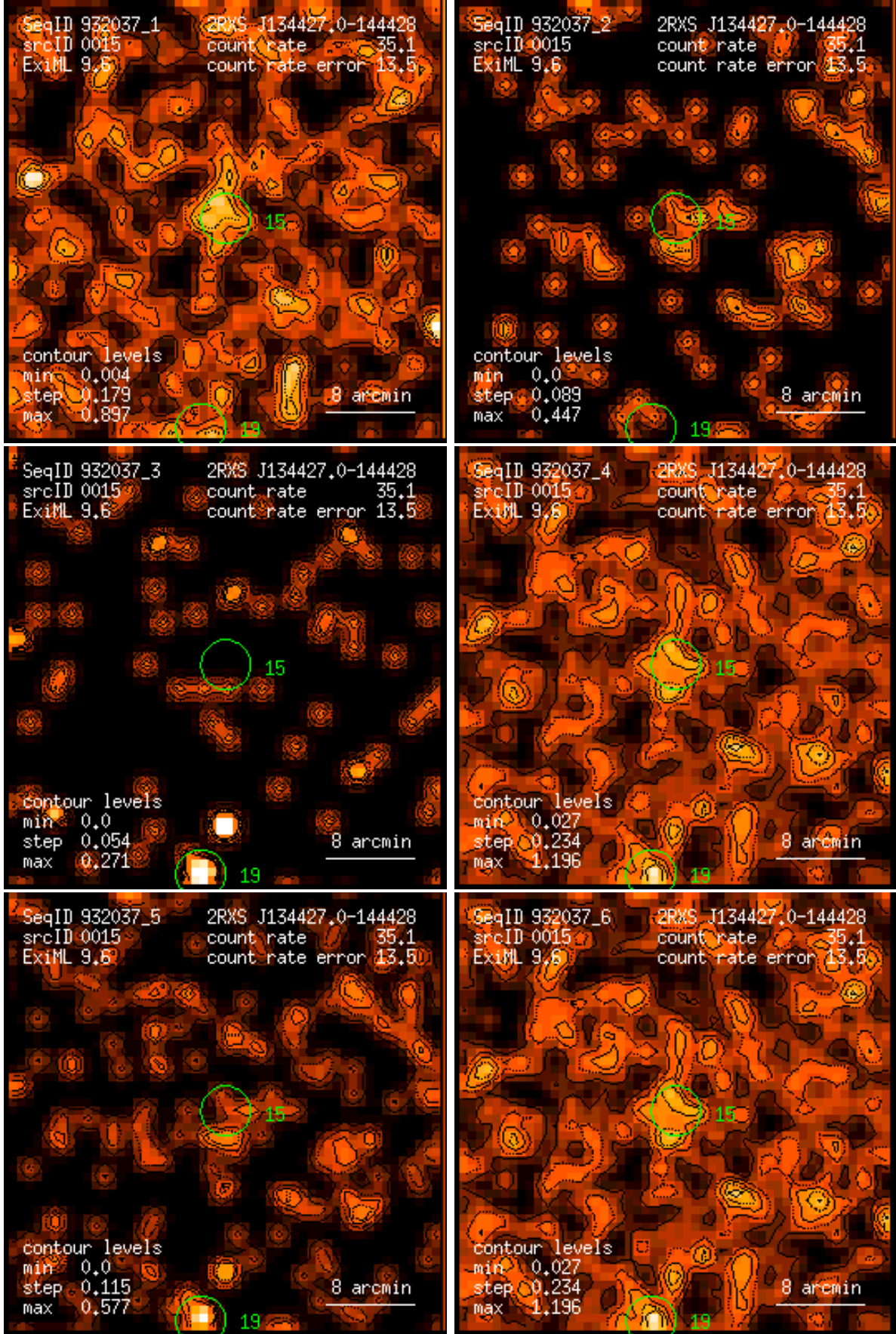
Figure 15: RASS 932037: detection 0015: band rate images, Gaussian filter: (1) PSPC channels 11 – 41, (2) 52 – 90, (3) 91 – 201, (4) 11 – 235, (5) 52 – 201, (6) 11 – 201. Broad band rates in counts/ks. Band rate contour levels in counts/ks/arcmin 2 .
