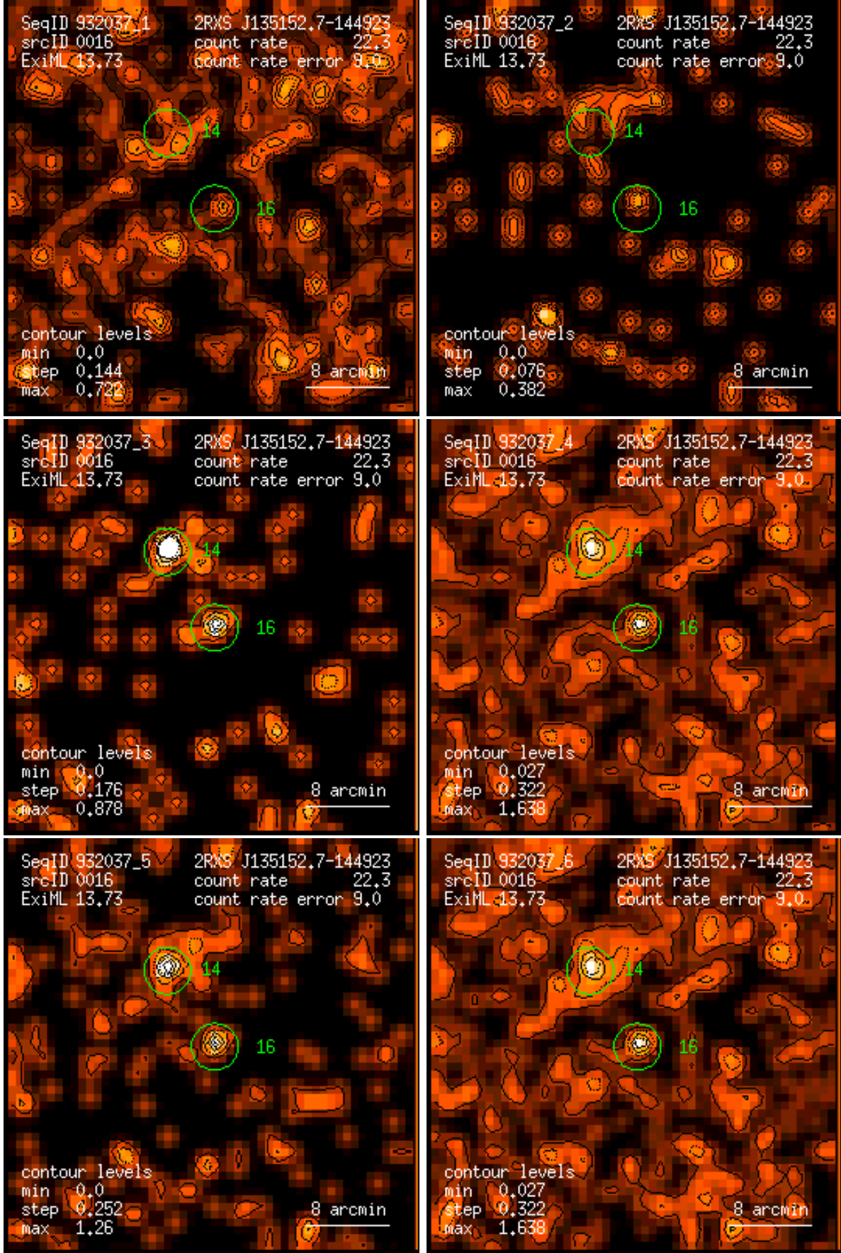
Figure 16: RASS 932037: detection 0016: band rate images, Gaussian filter: (1) PSPC channels 11 – 41, (2) 52 – 90, (3) 91 – 201, (4) 11 – 235, (5) 52 – 201, (6) 11 – 201. Broad band rates in counts/ks. Band rate contour levels in counts/ks/arcmin 2 .
