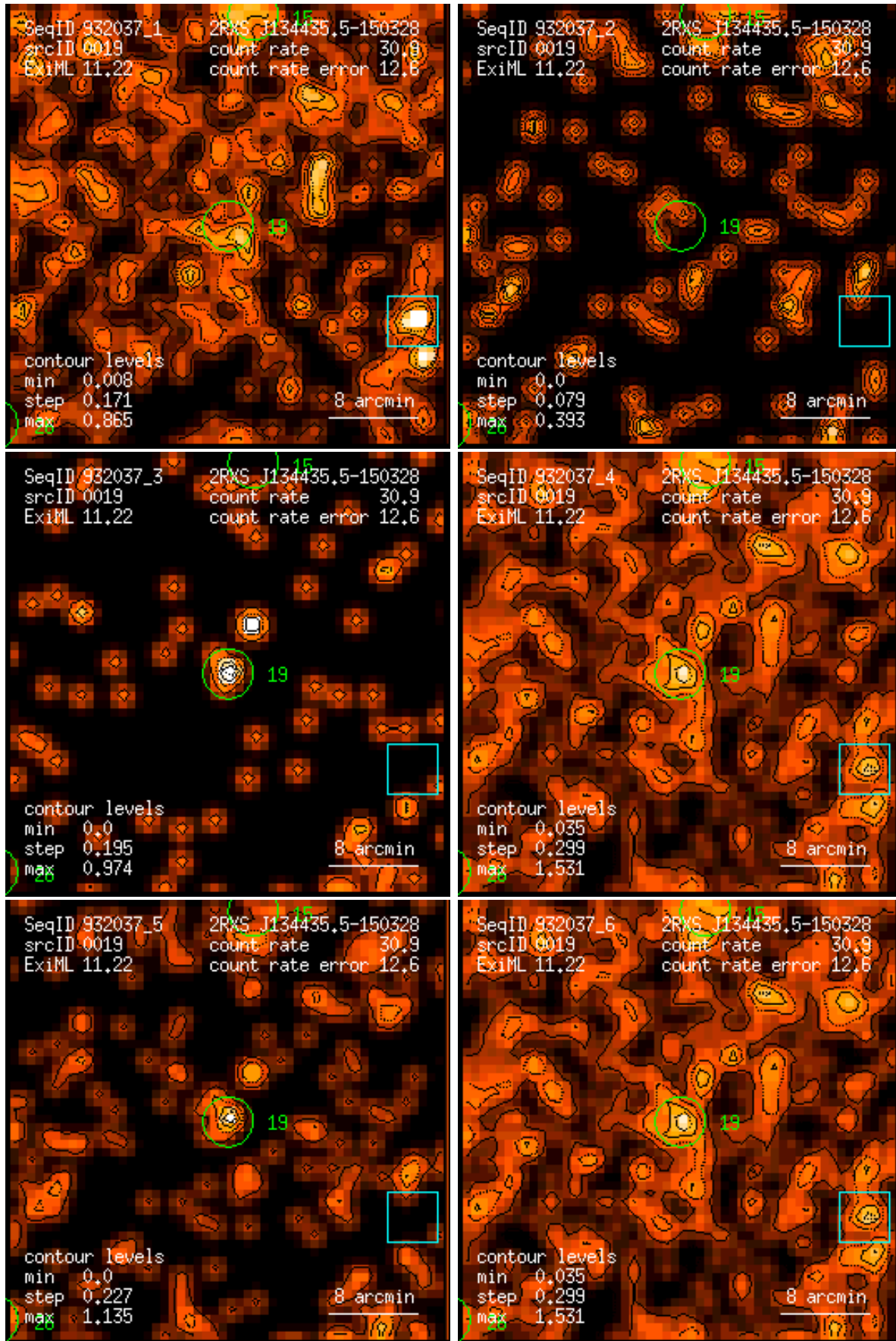
Figure 19: RASS 932037: detection 0019: band rate images, Gaussian filter: (1) PSPC channels 11 – 41, (2) 52 – 90, (3) 91 – 201, (4) 11 – 235, (5) 52 – 201, (6) 11 – 201. Broad band rates in counts/ks. Band rate contour levels in counts/ks/arcmin 2 .
