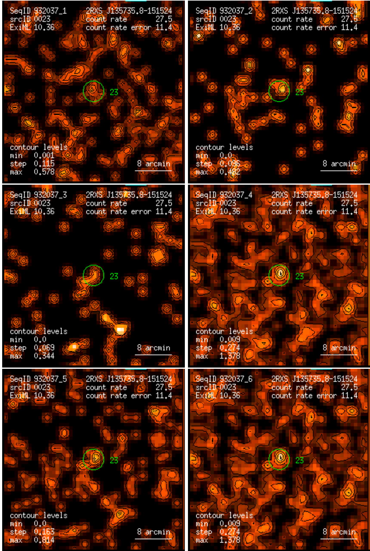
Figure 23: RASS 932037: detection 0023: band rate images, Gaussian filter: (1) PSPC channels 11 – 41, (2) 52 – 90, (3) 91 – 201, (4) 11 – 235, (5) 52 – 201, (6) 11 – 201. Broad band rates in counts/ks. Band rate contour levels in counts/ks/arcmin 2 .
