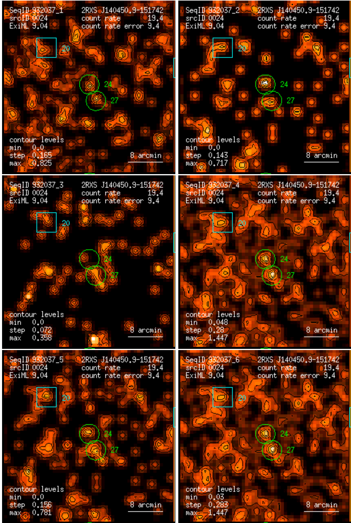
Figure 24: RASS 932037: detection 0024: band rate images, Gaussian filter: (1) PSPC channels 11 – 41, (2) 52 – 90, (3) 91 – 201, (4) 11 – 235, (5) 52 – 201, (6) 11 – 201. Broad band rates in counts/ks. Band rate contour levels in counts/ks/arcmin 2 .
