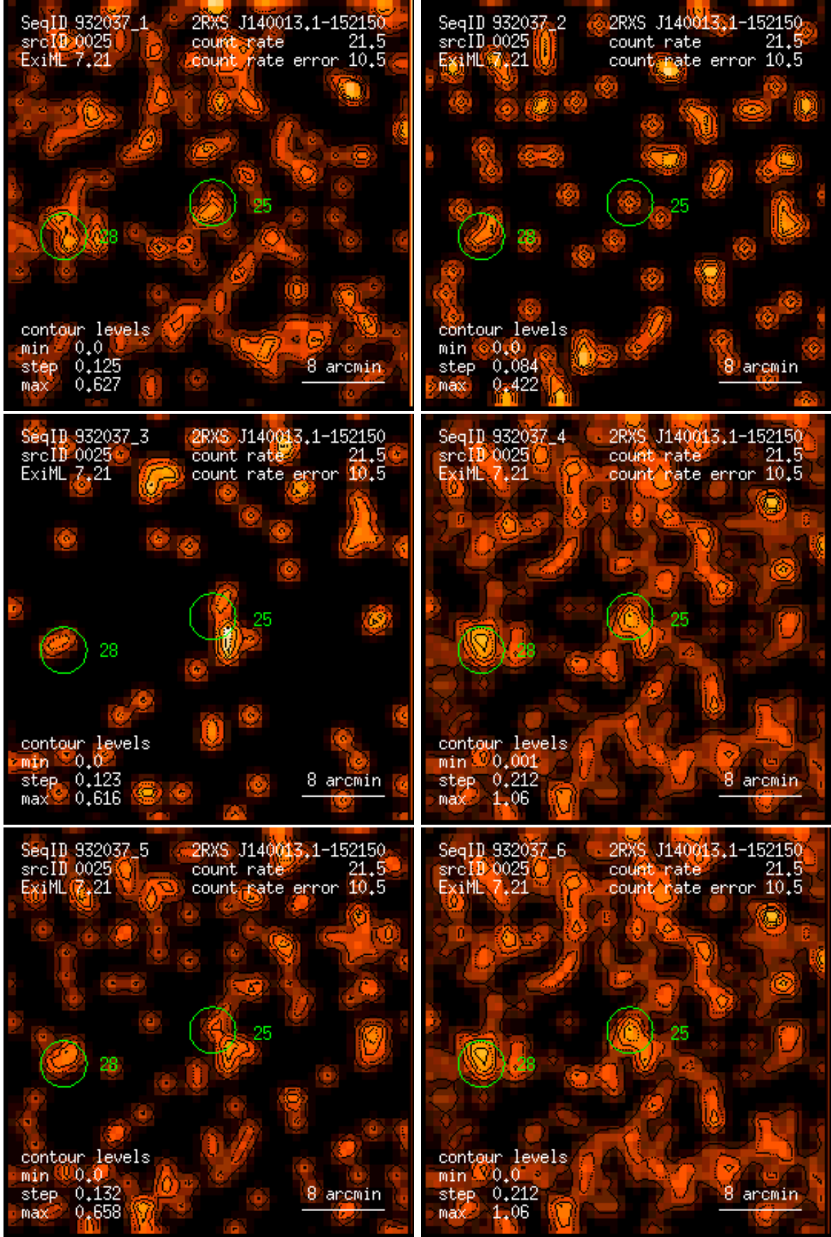
Figure 25: RASS 932037: detection 0025: band rate images, Gaussian filter: (1) PSPC channels 11 – 41, (2) 52 – 90, (3) 91 – 201, (4) 11 – 235, (5) 52 – 201, (6) 11 – 201. Broad band rates in counts/ks. Band rate contour levels in counts/ks/arcmin 2 .
