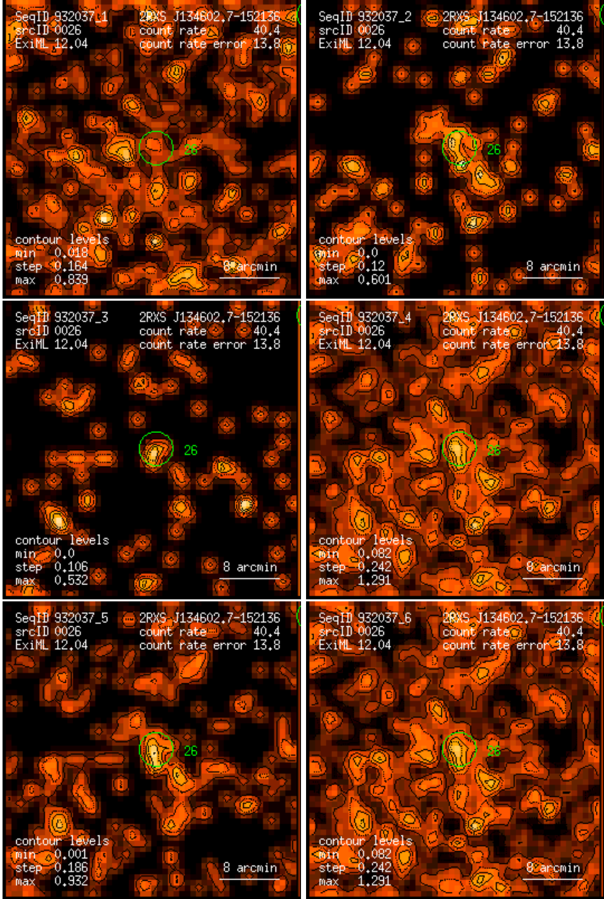
Figure 26: RASS 932037: detection 0026: band rate images, Gaussian filter: (1) PSPC channels 11 – 41, (2) 52 – 90, (3) 91 – 201, (4) 11 – 235, (5) 52 – 201, (6) 11 – 201. Broad band rates in counts/ks. Band rate contour levels in counts/ks/arcmin 2 .
