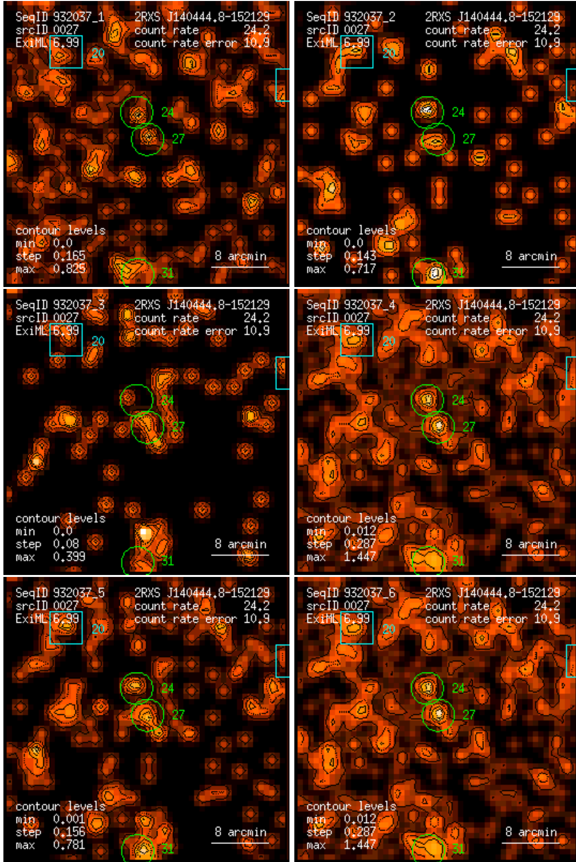
Figure 27: RASS 932037: detection 0027: band rate images, Gaussian filter: (1) PSPC channels 11 – 41, (2) 52 – 90, (3) 91 – 201, (4) 11 – 235, (5) 52 – 201, (6) 11 – 201. Broad band rates in counts/ks. Band rate contour levels in counts/ks/arcmin 2 .
