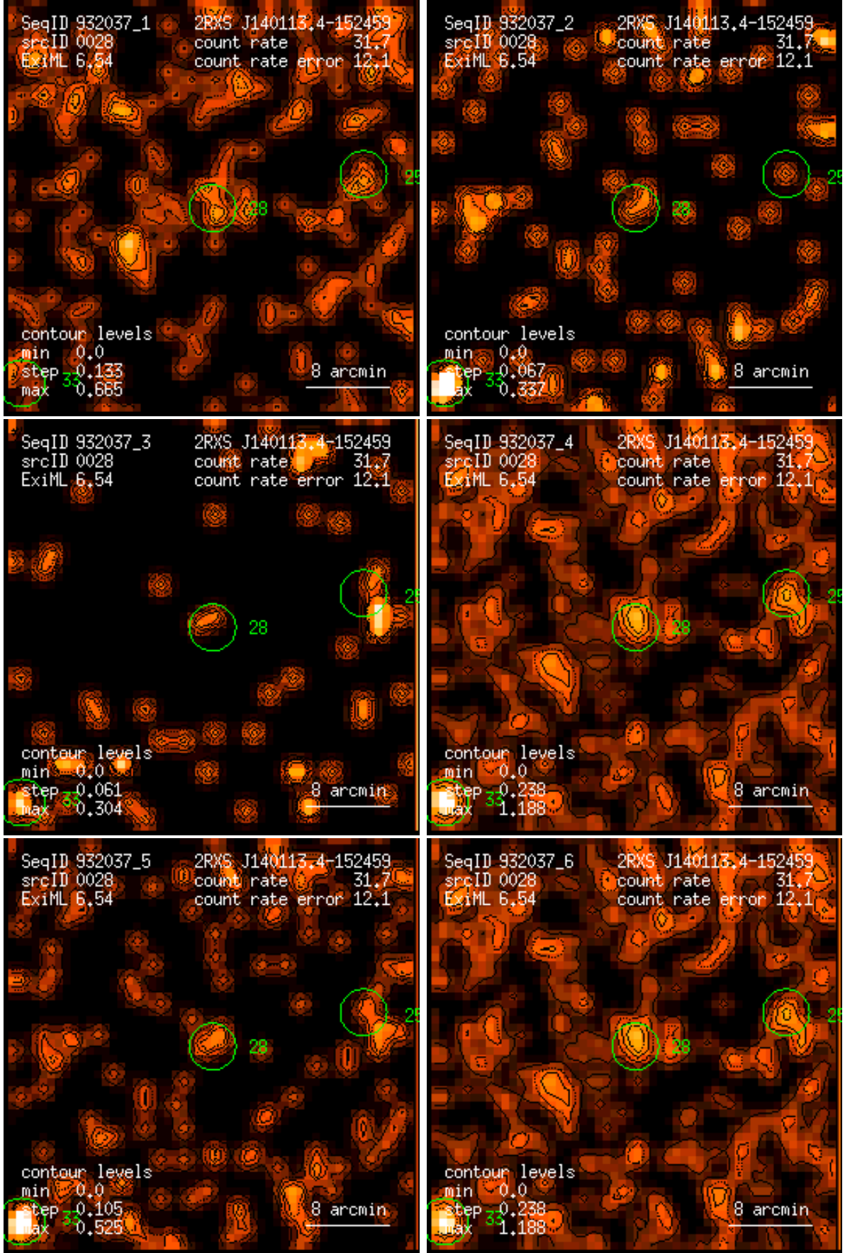
Figure 28: RASS 932037: detection 0028: band rate images, Gaussian filter: (1) PSPC channels 11 – 41, (2) 52 – 90, (3) 91 – 201, (4) 11 – 235, (5) 52 – 201, (6) 11 – 201. Broad band rates in counts/ks. Band rate contour levels in counts/ks/arcmin 2 .
