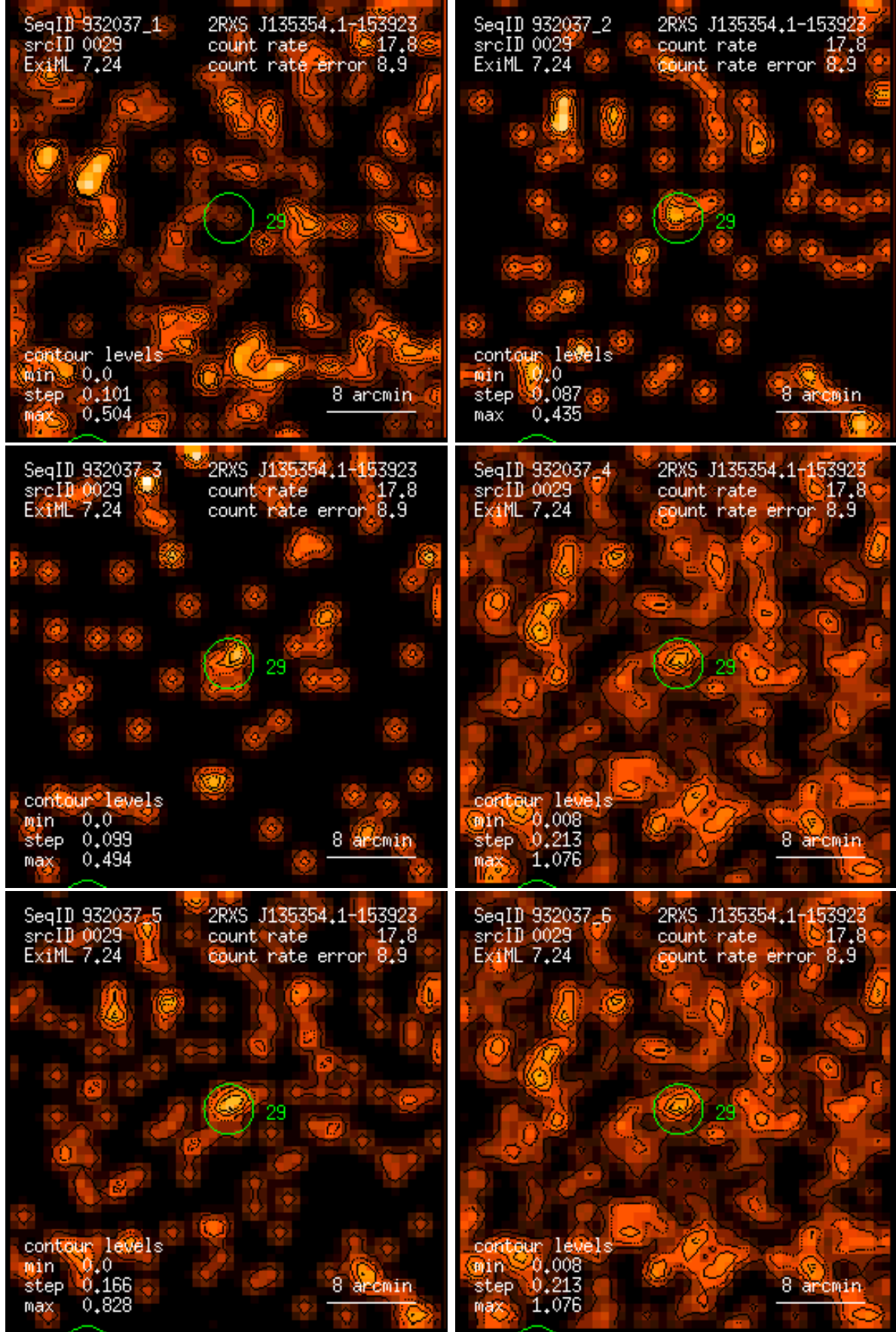
Figure 29: RASS 932037: detection 0029: band rate images, Gaussian filter: (1) PSPC channels 11 – 41, (2) 52 – 90, (3) 91 – 201, (4) 11 – 235, (5) 52 – 201, (6) 11 – 201. Broad band rates in counts/ks. Band rate contour levels in counts/ks/arcmin 2 .
