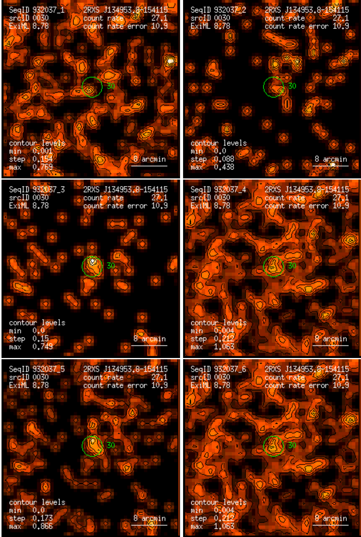
Figure 30: RASS 932037: detection 0030: band rate images, Gaussian filter: (1) PSPC channels 11 – 41, (2) 52 – 90, (3) 91 – 201, (4) 11 – 235, (5) 52 – 201, (6) 11 – 201. Broad band rates in counts/ks. Band rate contour levels in counts/ks/arcmin 2 .
