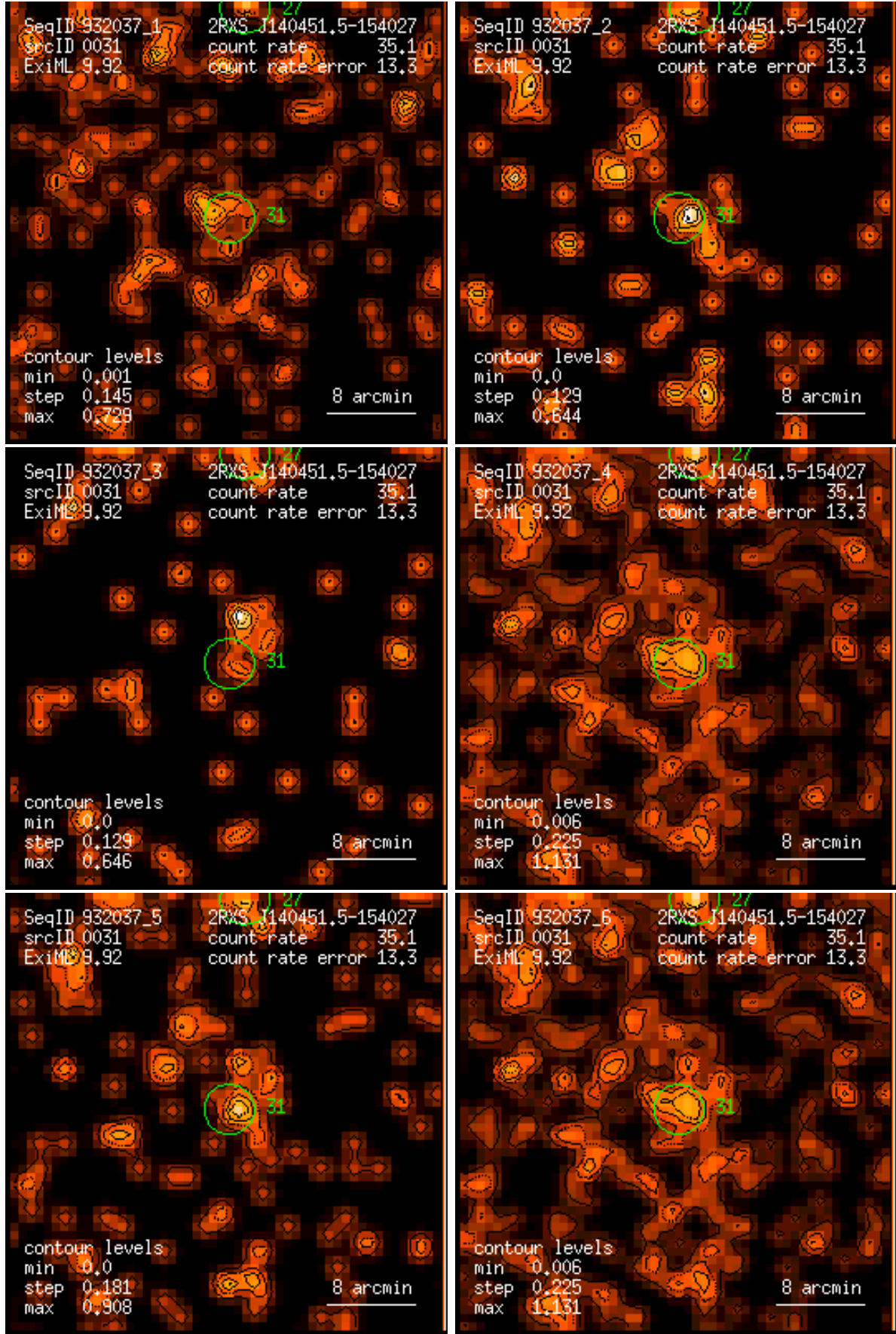
Figure 31: RASS 932037: detection 0031: band rate images, Gaussian filter: (1) PSPC channels 11 – 41, (2) 52 – 90, (3) 91 – 201, (4) 11 – 235, (5) 52 – 201, (6) 11 – 201. Broad band rates in counts/ks. Band rate contour levels in counts/ks/arcmin 2 .
