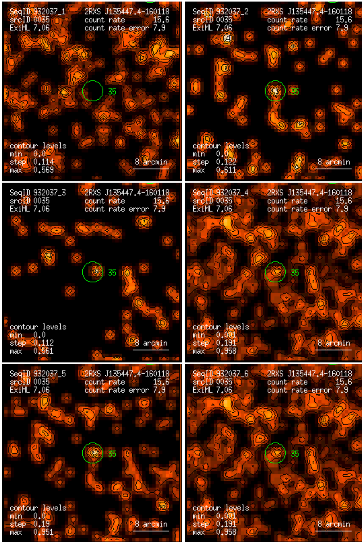
Figure 35: RASS 932037: detection 0035: band rate images, Gaussian filter: (1) PSPC channels 11 – 41, (2) 52 – 90, (3) 91 – 201, (4) 11 – 235, (5) 52 – 201, (6) 11 – 201. Broad band rates in counts/ks. Band rate contour levels in counts/ks/arcmin 2 .
