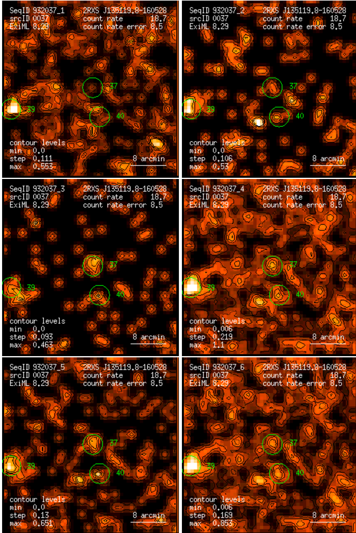
Figure 37: RASS 932037: detection 0037: band rate images, Gaussian filter: (1) PSPC channels 11 – 41, (2) 52 – 90, (3) 91 – 201, (4) 11 – 235, (5) 52 – 201, (6) 11 – 201. Broad band rates in counts/ks. Band rate contour levels in counts/ks/arcmin 2 .
