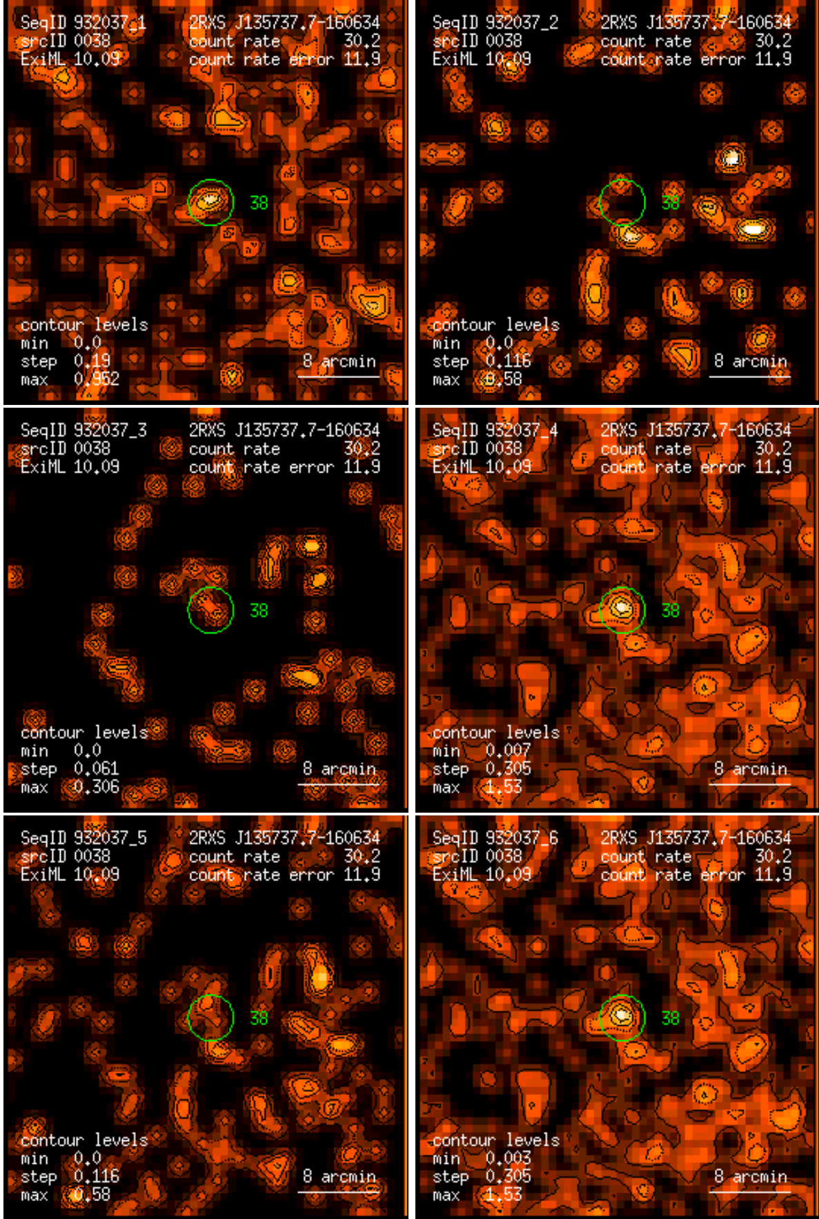
Figure 38: RASS 932037: detection 0038: band rate images, Gaussian filter: (1) PSPC channels 11 – 41, (2) 52 – 90, (3) 91 – 201, (4) 11 – 235, (5) 52 – 201, (6) 11 – 201. Broad band rates in counts/ks. Band rate contour levels in counts/ks/arcmin 2 .
