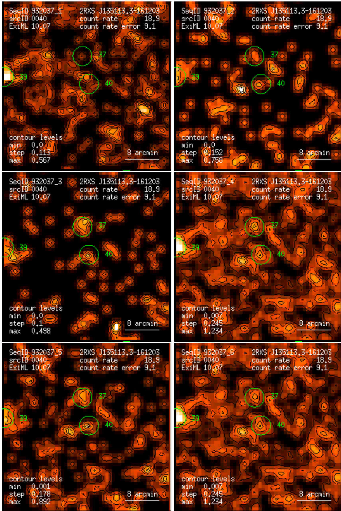
Figure 40: RASS 932037: detection 0040: band rate images, Gaussian filter: (1) PSPC channels 11 – 41, (2) 52 – 90, (3) 91 – 201, (4) 11 – 235, (5) 52 – 201, (6) 11 – 201. Broad band rates in counts/ks. Band rate contour levels in counts/ks/arcmin 2 .
