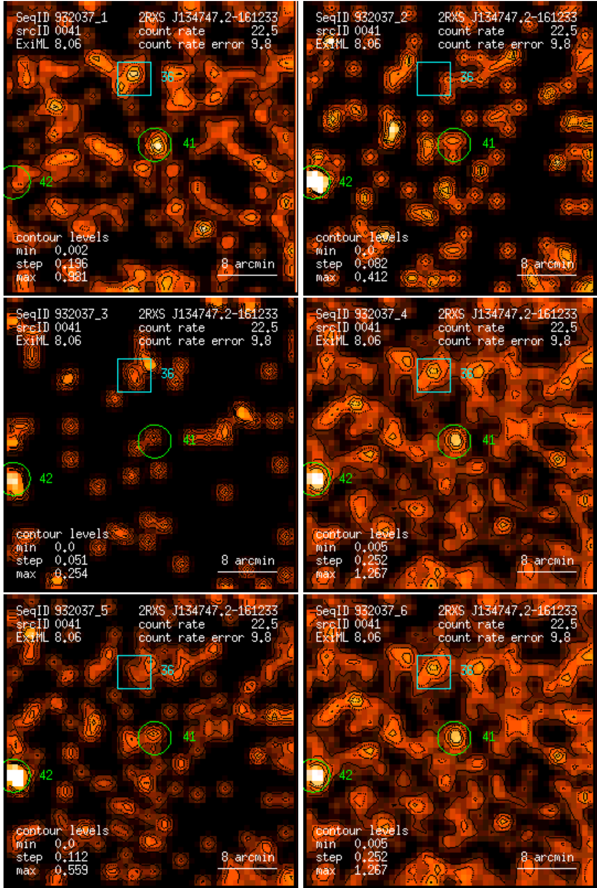
Figure 41: RASS 932037: detection 0041: band rate images, Gaussian filter: (1) PSPC channels 11 – 41, (2) 52 – 90, (3) 91 – 201, (4) 11 – 235, (5) 52 – 201, (6) 11 – 201. Broad band rates in counts/ks. Band rate contour levels in counts/ks/arcmin 2 .
