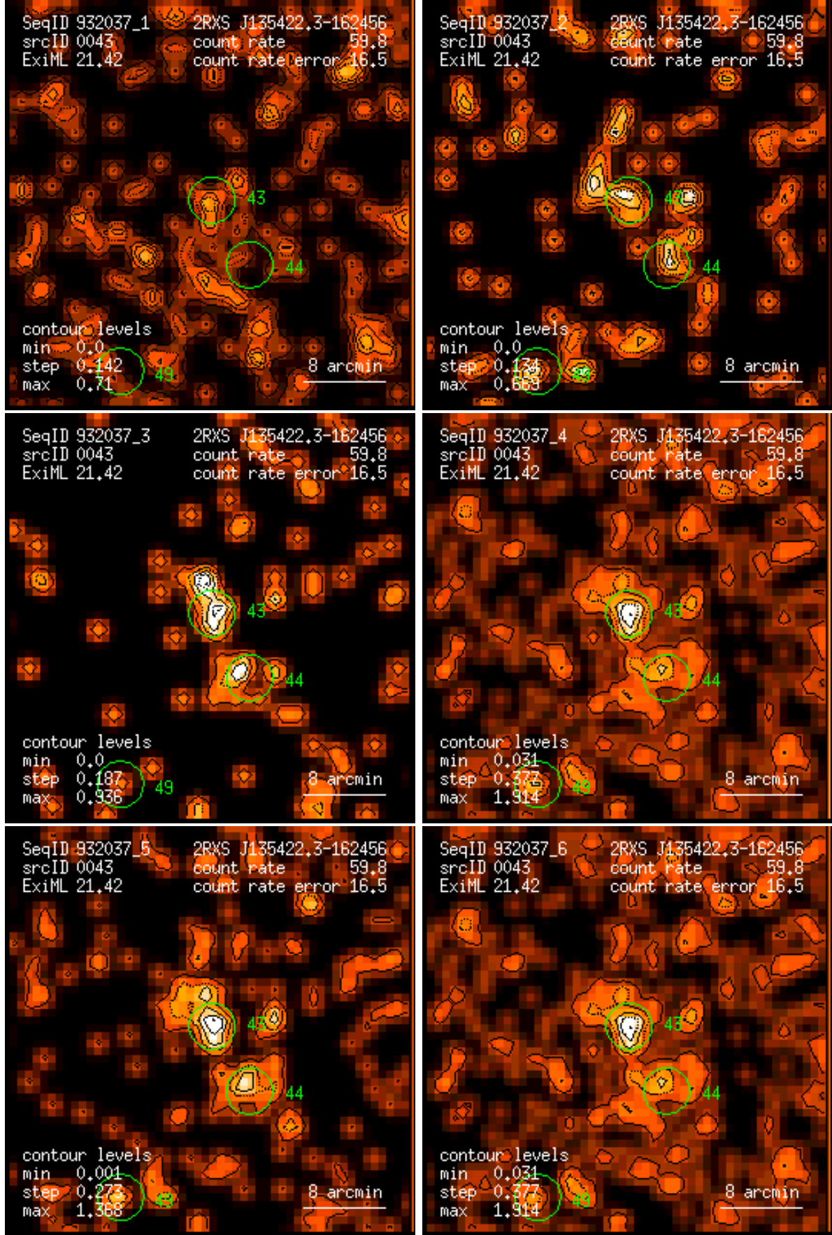
Figure 43: RASS 932037: detection 0043: band rate images, Gaussian filter: (1) PSPC channels 11 – 41, (2) 52 – 90, (3) 91 – 201, (4) 11 – 235, (5) 52 – 201, (6) 11 – 201. Broad band rates in counts/ks. Band rate contour levels in counts/ks/arcmin 2 .
