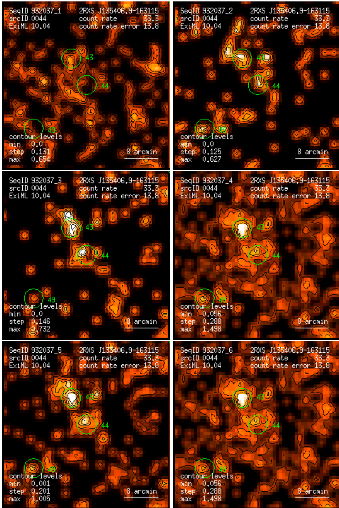
Figure 44: RASS 932037: detection 0044: band rate images, Gaussian filter: (1) PSPC channels 11 – 41, (2) 52 – 90, (3) 91 – 201, (4) 11 – 235, (5) 52 – 201, (6) 11 – 201. Broad band rates in counts/ks. Band rate contour levels in counts/ks/arcmin 2 .
