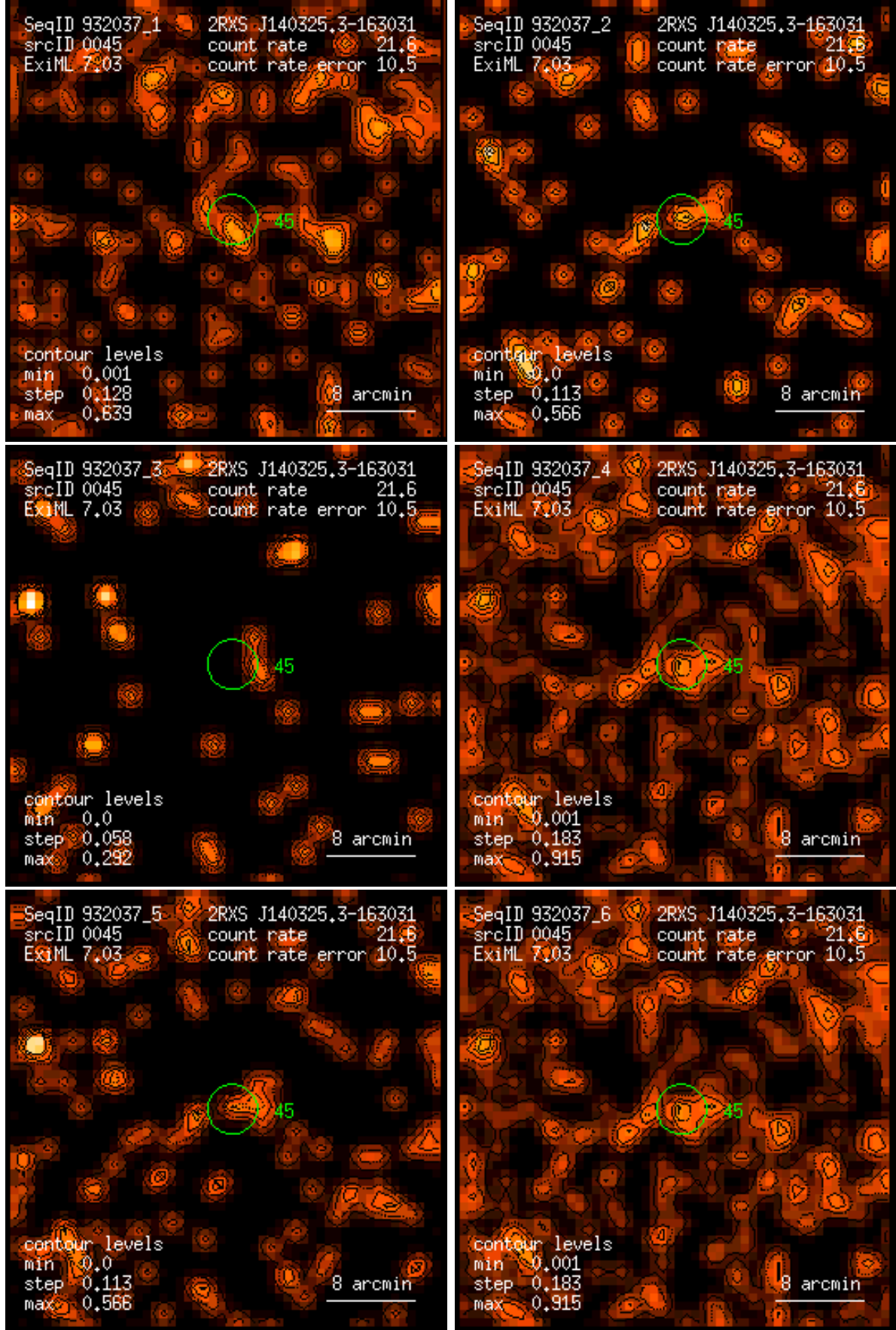
Figure 45: RASS 932037: detection 0045: band rate images, Gaussian filter: (1) PSPC channels 11 – 41, (2) 52 – 90, (3) 91 – 201, (4) 11 – 235, (5) 52 – 201, (6) 11 – 201. Broad band rates in counts/ks. Band rate contour levels in counts/ks/arcmin 2 .
