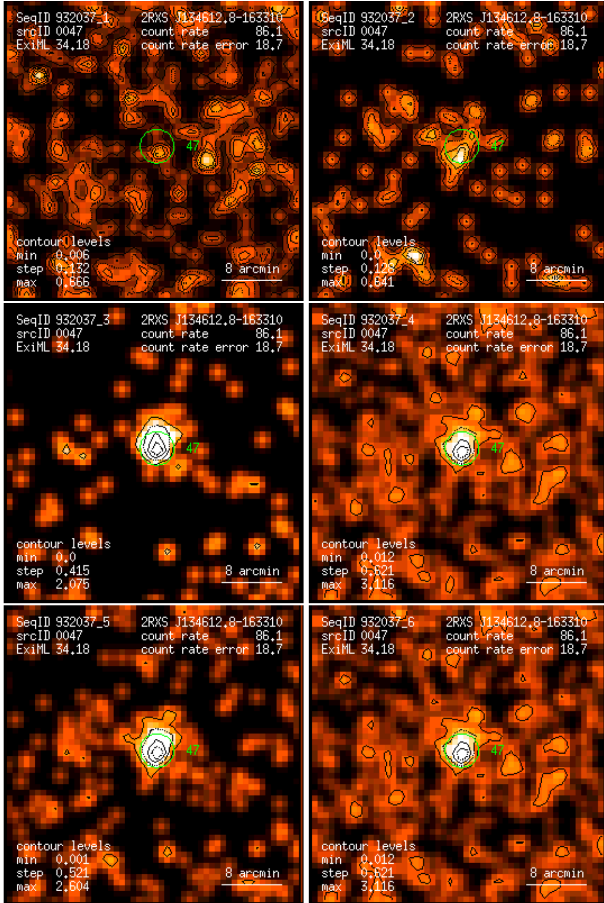
Figure 47: RASS 932037: detection 0047: band rate images, Gaussian filter: (1) PSPC channels 11 – 41, (2) 52 – 90, (3) 91 – 201, (4) 11 – 235, (5) 52 – 201, (6) 11 – 201. Broad band rates in counts/ks. Band rate contour levels in counts/ks/arcmin 2 .
