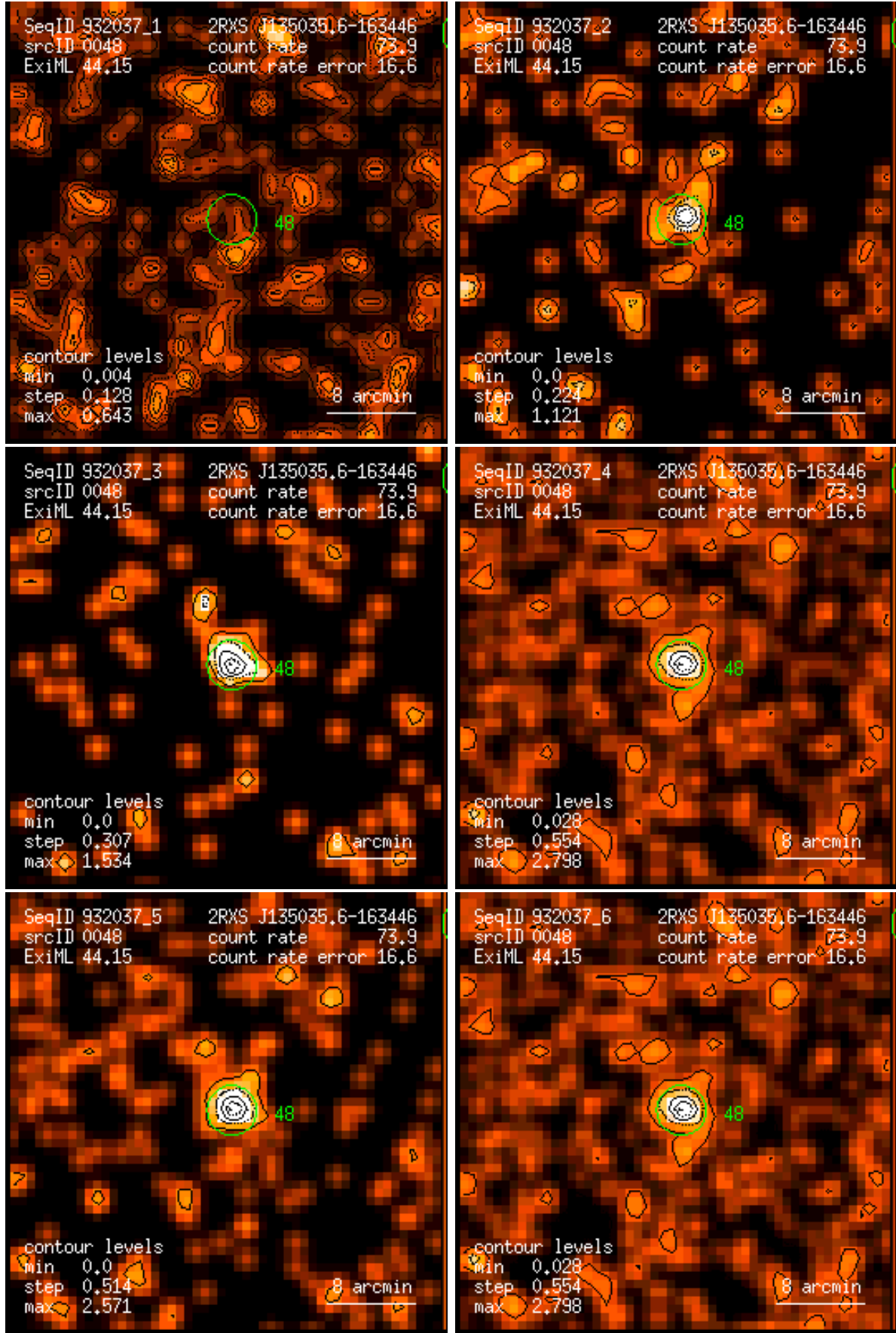
Figure 48: RASS 932037: detection 0048: band rate images, Gaussian filter: (1) PSPC channels 11 – 41, (2) 52 – 90, (3) 91 – 201, (4) 11 – 235, (5) 52 – 201, (6) 11 – 201. Broad band rates in counts/ks. Band rate contour levels in counts/ks/arcmin 2 .
