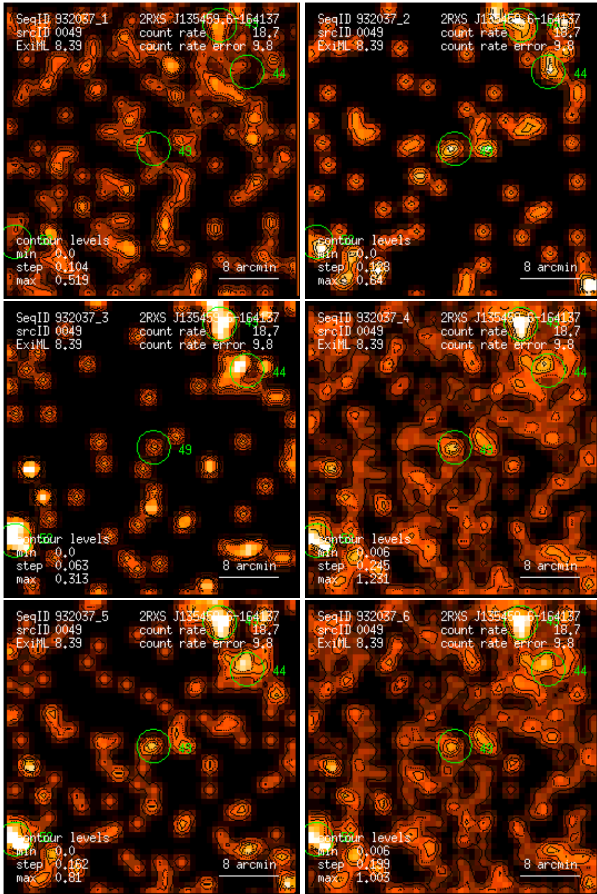
Figure 49: RASS 932037: detection 0049: band rate images, Gaussian filter: (1) PSPC channels 11 – 41, (2) 52 – 90, (3) 91 – 201, (4) 11 – 235, (5) 52 – 201, (6) 11 – 201. Broad band rates in counts/ks. Band rate contour levels in counts/ks/arcmin 2 .
