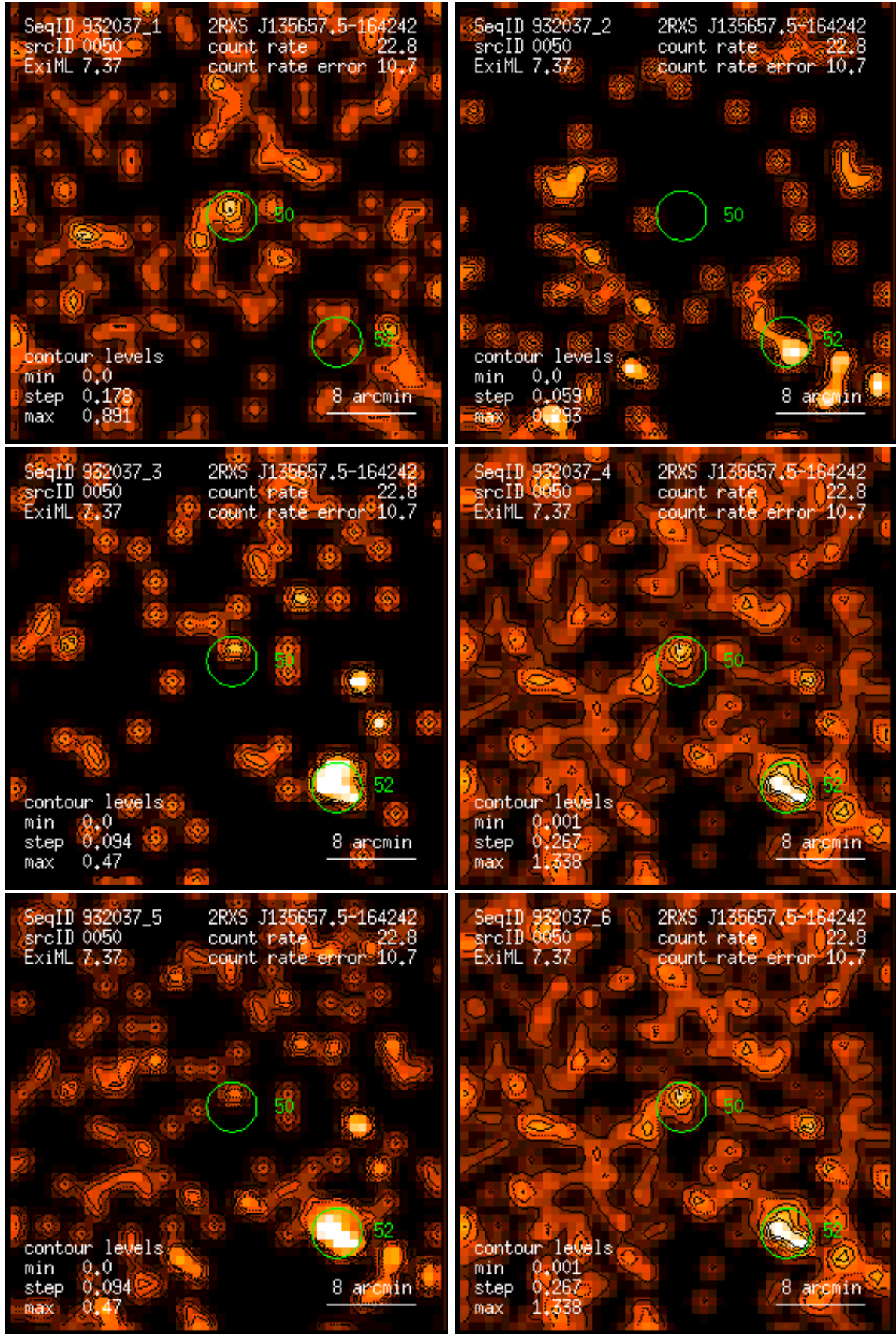
Figure 50: RASS 932037: detection 0050: band rate images, Gaussian filter: (1) PSPC channels 11 – 41, (2) 52 – 90, (3) 91 – 201, (4) 11 – 235, (5) 52 – 201, (6) 11 – 201. Broad band rates in counts/ks. Band rate contour levels in counts/ks/arcmin 2 .
