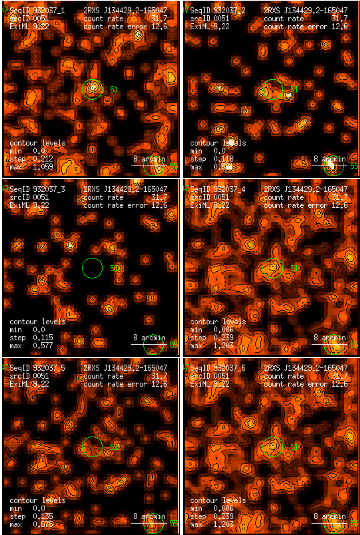
Figure 51: RASS 932037: detection 0051: band rate images, Gaussian filter: (1) PSPC channels 11 – 41, (2) 52 – 90, (3) 91 – 201, (4) 11 – 235, (5) 52 – 201, (6) 11 – 201. Broad band rates in counts/ks. Band rate contour levels in counts/ks/arcmin 2 .
