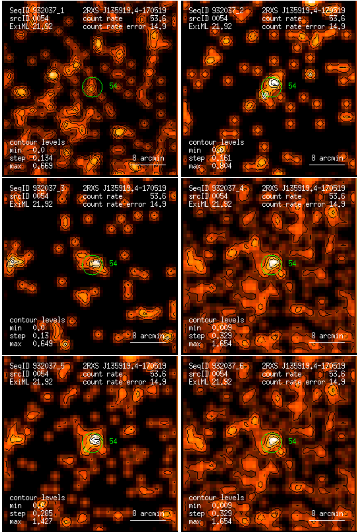
Figure 54: RASS 932037: detection 0054: band rate images, Gaussian filter: (1) PSPC channels 11 – 41, (2) 52 – 90, (3) 91 – 201, (4) 11 – 235, (5) 52 – 201, (6) 11 – 201. Broad band rates in counts/ks. Band rate contour levels in counts/ks/arcmin 2 .
