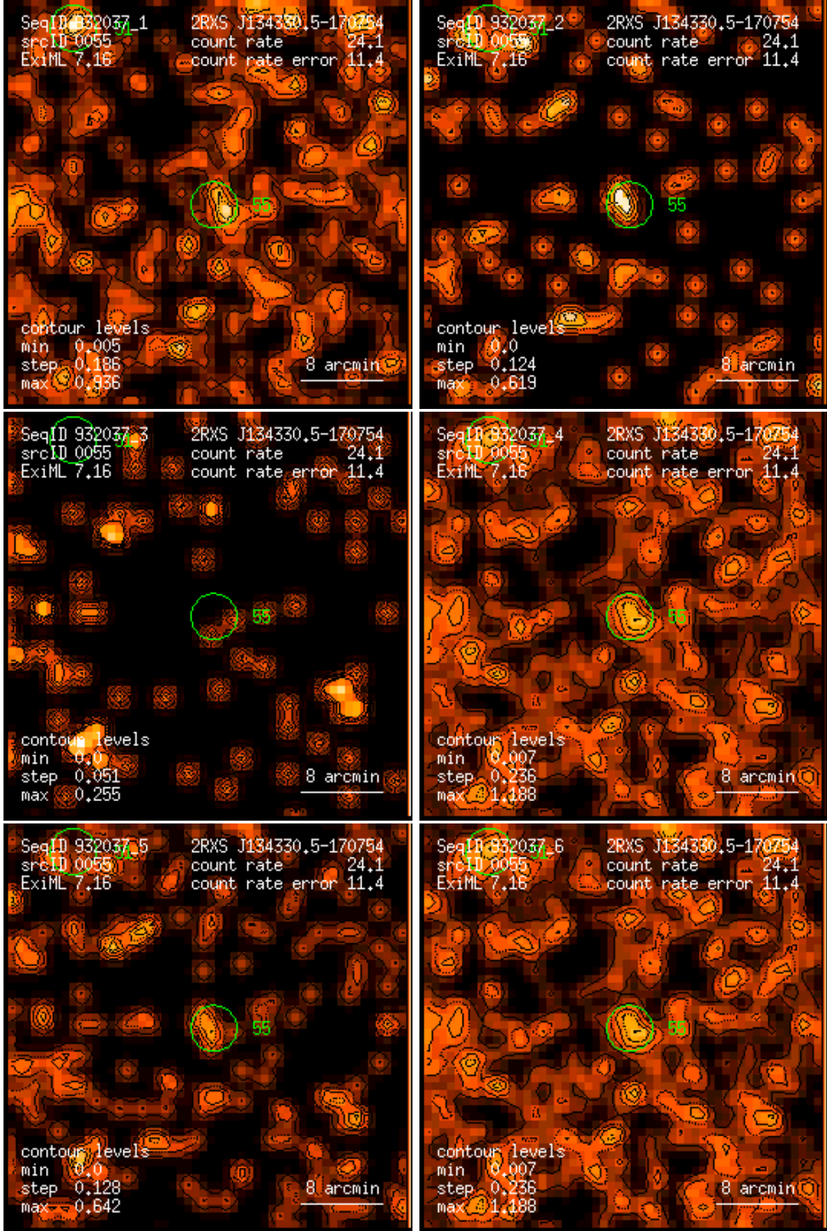
Figure 55: RASS 932037: detection 0055: band rate images, Gaussian filter: (1) PSPC channels 11 – 41, (2) 52 – 90, (3) 91 – 201, (4) 11 – 235, (5) 52 – 201, (6) 11 – 201. Broad band rates in counts/ks. Band rate contour levels in counts/ks/arcmin 2 .
