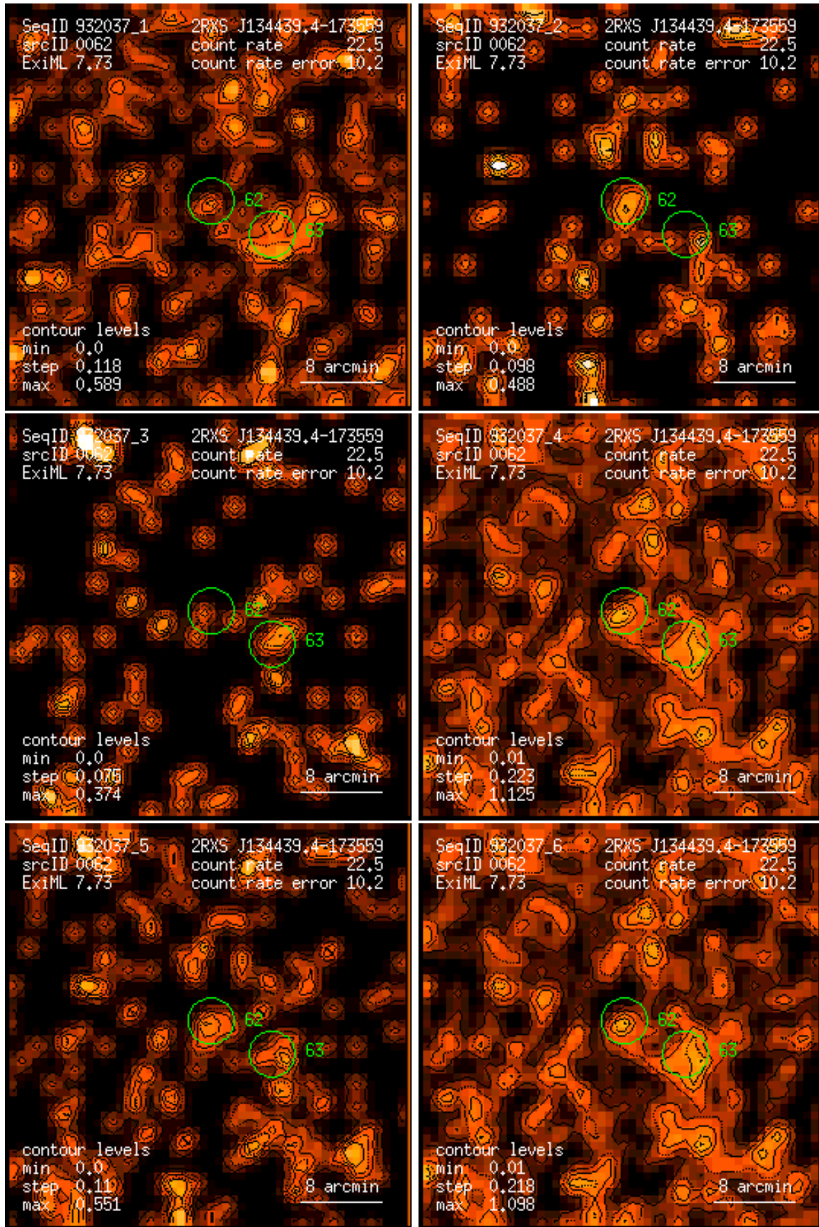
Figure 62: RASS 932037: detection 0062: band rate images, Gaussian filter: (1) PSPC channels 11 – 41, (2) 52 – 90, (3) 91 – 201, (4) 11 – 235, (5) 52 – 201, (6) 11 – 201. Broad band rates in counts/ks. Band rate contour levels in counts/ks/arcmin 2 .
