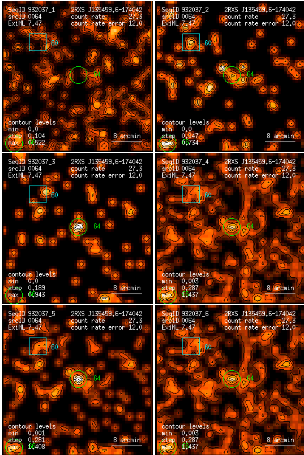
Figure 64: RASS 932037: detection 0064: band rate images, Gaussian filter: (1) PSPC channels 11 – 41, (2) 52 – 90, (3) 91 – 201, (4) 11 – 235, (5) 52 – 201, (6) 11 – 201. Broad band rates in counts/ks. Band rate contour levels in counts/ks/arcmin 2 .
