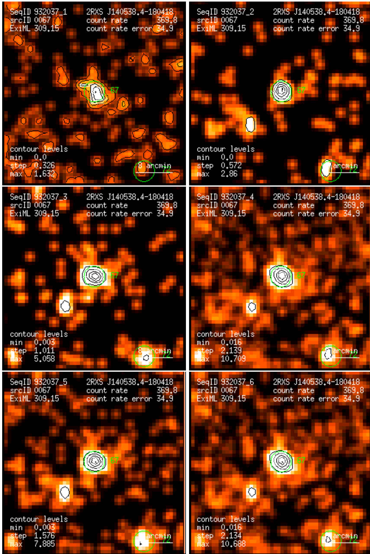
Figure 67: RASS 932037: detection 0067: band rate images, Gaussian filter: (1) PSPC channels 11 – 41, (2) 52 – 90, (3) 91 – 201, (4) 11 – 235, (5) 52 – 201, (6) 11 – 201. Broad band rates in counts/ks. Band rate contour levels in counts/ks/arcmin 2 .
