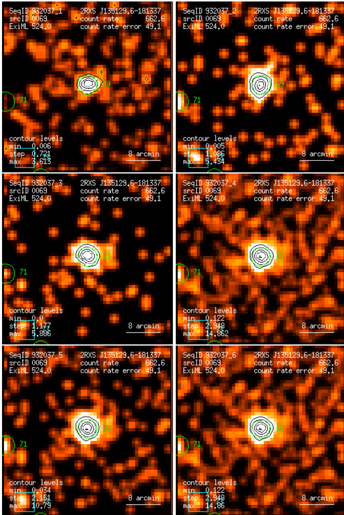
Figure 69: RASS 932037: detection 0069: band rate images, Gaussian filter: (1) PSPC channels 11 – 41, (2) 52 – 90, (3) 91 – 201, (4) 11 – 235, (5) 52 – 201, (6) 11 – 201. Broad band rates in counts/ks. Band rate contour levels in counts/ks/arcmin 2 .
