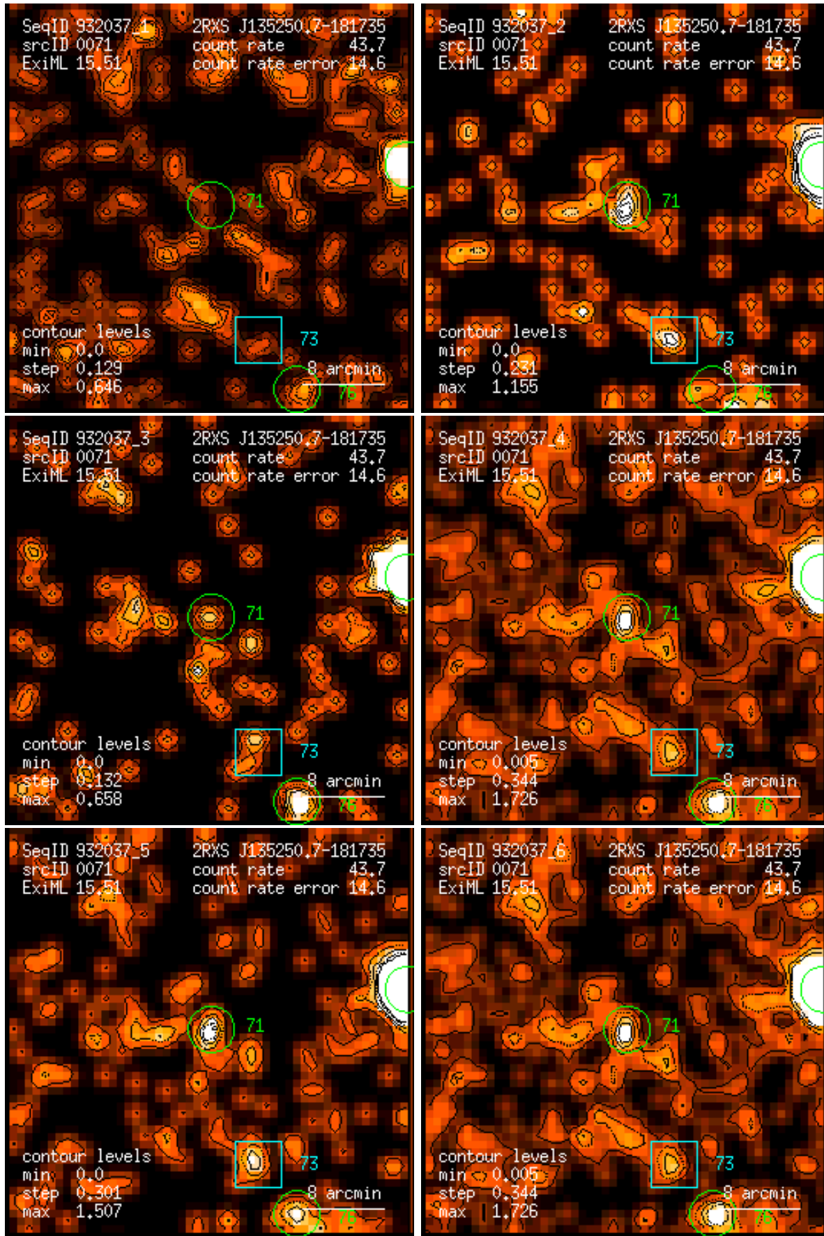
Figure 71: RASS 932037: detection 0071: band rate images, Gaussian filter: (1) PSPC channels 11 – 41, (2) 52 – 90, (3) 91 – 201, (4) 11 – 235, (5) 52 – 201, (6) 11 – 201. Broad band rates in counts/ks. Band rate contour levels in counts/ks/arcmin 2 .
