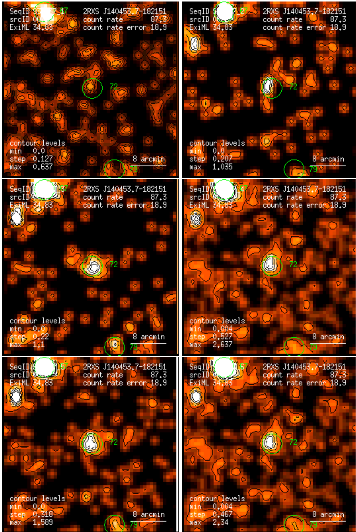
Figure 72: RASS 932037: detection 0072: band rate images, Gaussian filter: (1) PSPC channels 11 – 41, (2) 52 – 90, (3) 91 – 201, (4) 11 – 235, (5) 52 – 201, (6) 11 – 201. Broad band rates in counts/ks. Band rate contour levels in counts/ks/arcmin 2 .
